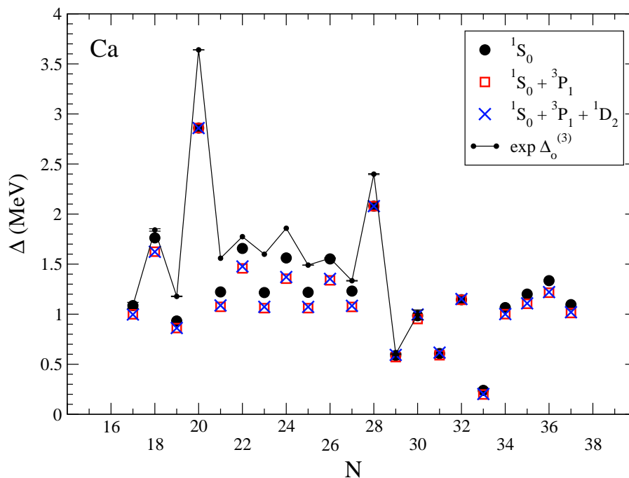
Figure 3. (Color online) Same as Fig. 1, but for calcium isotopes.
