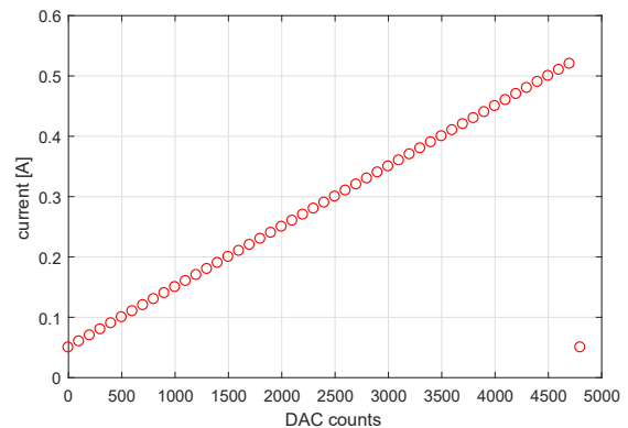
Figure 5: The over-current event triggered on the chosen output channel with short applied.
