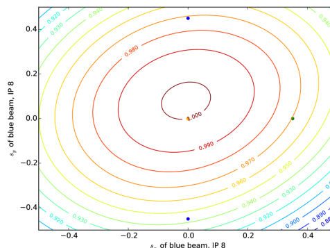
Figure 4: The luminosity reduction as function of the s_H^* and s_V^* of the blue beam. The requested s_V^* change is marked with blue dots; the requested s_H^* is marked with green dot and the origin s^* is marked yellow dot.
