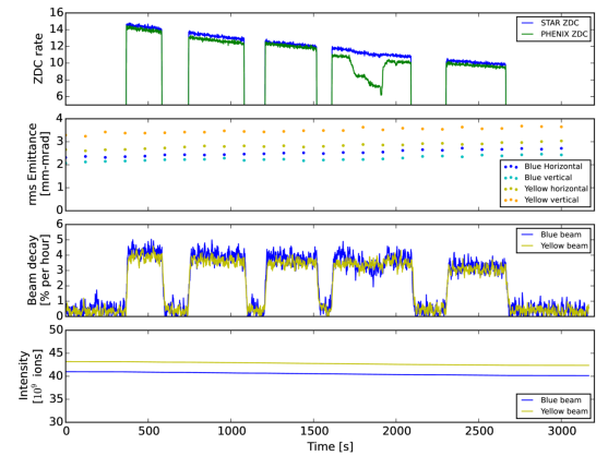
Figure 2: From top figures to the bottom: first: The ZDC rate of the STAR and PHENIX detector; second: the rms emittance of the two colliding beam in two transverse directions; third: the bunch decay rate of both beams; fourth: the bunch intensity of both beams.
