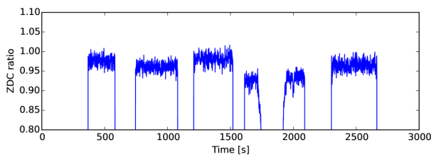
Figure 3: The ZDC rate ratio, defined as the PHENIX ZDC rate divided by the STAR ZDC rate.
