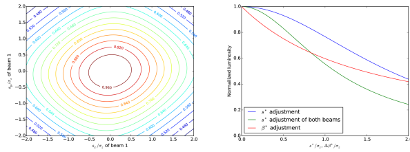
Figure 1: Top: The luminosity control contour due to the waist position adjustment of beam 1. The waist position of the other beam is intact. Bottom: The residue luminosity comparison of s^* tuning of one beam and \beta^* tuning of both beams, the s_x^* = s_y^* = s^* and \Delta\beta^* is the beta function tuning amplitude. In both figures the luminosity is normalized by original luminosity with any adjustments.
