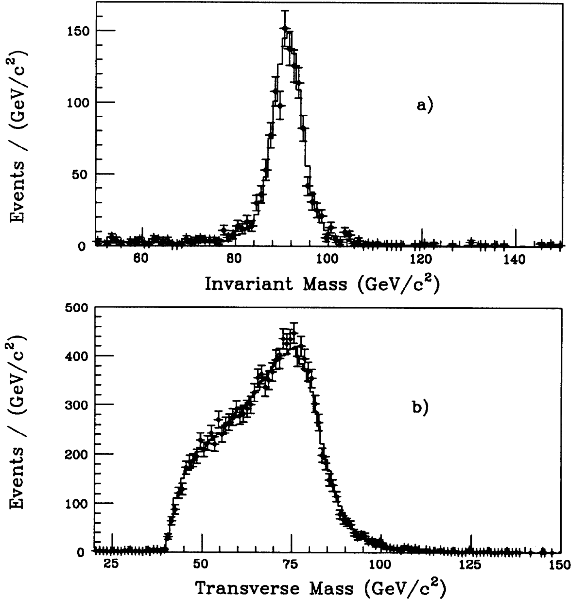
Figure 1: (a) Observed distribution of invariant mass of e^+e^- pairs satisfying our electron selection criteria. Z^0 candidates are taken to lie in the range 66 - 116 \text{ GeV}/c^2 . (b) Observed distribution of transverse mass of the W candidates. The curves in both plots are the sum of the expected background shape and the predicted spectrum from the Monte Carlo used in the acceptance calculation.
