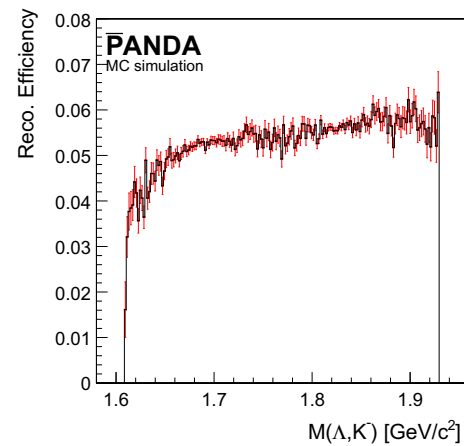
Fig. 11 Reconstruction efficiency (black histogram) as function of the invariant \Lambda K^- mass in the process \bar{p}p \rightarrow \Xi^+ \Lambda K^- . The statistical error is shown in red
