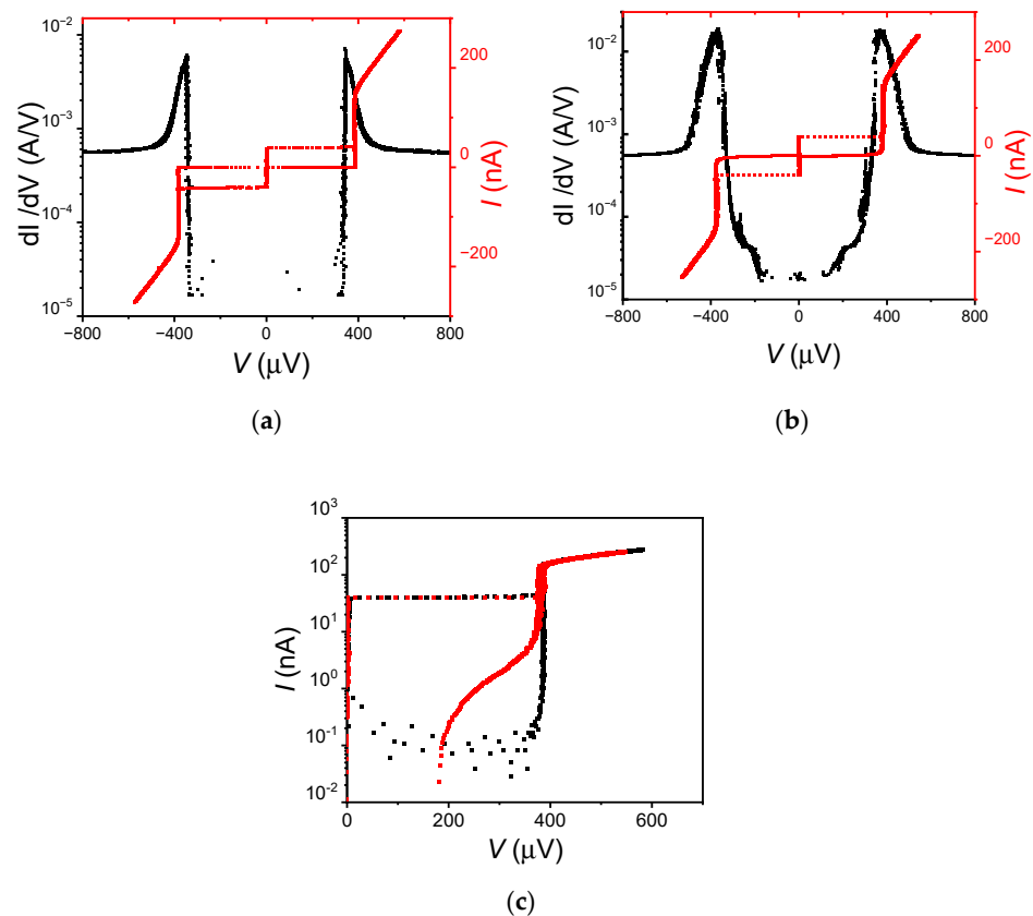
Figure 3. (a) Conductance dl/dV measurement and I–V curve for the SIS'S junction with a diameter of 4 \mu m; (b) conductance measurement and I–V curve for the SIS'FS junction with a diameter of 4 \mu m. The conductance measurements were performed by applying a magnetic field of 10 mT to suppress the Josephson supercurrent. (c) Magnification of the positive part branch of the I–V curve in a log-scale for both the SIS'S (black curve) and the SIS'FS (red curve) junction with a diameter of 4 \mu m.
