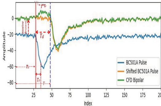
Fig 3: Digital pulse for BC501A and its CFD.
