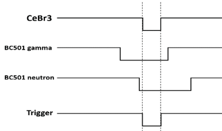
Fig 2: Timing Diagram for the Trigger.
