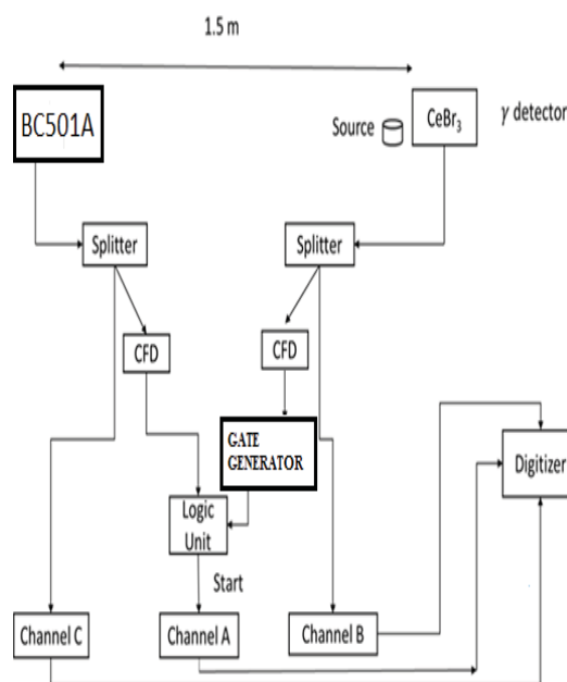
Fig.1: External trigger generation circuit for coincidence data collection.
