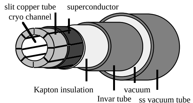
Figure 2: Conceptual sketch of superconducting transmission line.
