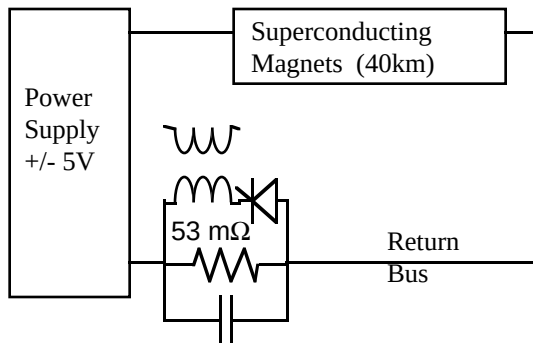
Figure 3: Power supply and quench protection cell.
