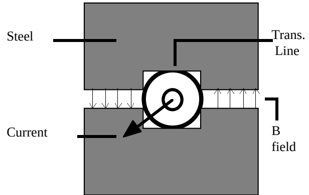
Figure 1: Conceptual sketch of superferric magnet powered by centrally located transmission line.
