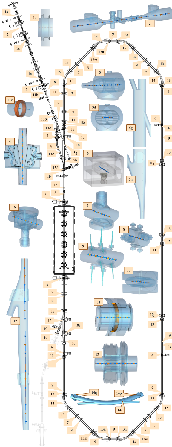
Figure 1 (above): Layout of bERLinPro with locations of various beam pipe insertions. Some components (1, 10, 11, 13) have similar sub-types, not all of them were analysed separately. Because of the limitations of the solver [2], only straight beam paths were computed.
