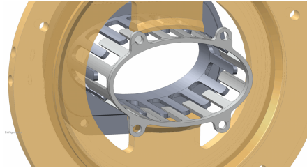
Figure 3: Internal design of the tunable bellow. The inner bars of the adjustable disc (ocher) between the bellow segments are extended close to the shielding fingers in order to enhance the tuning sensitivity.
