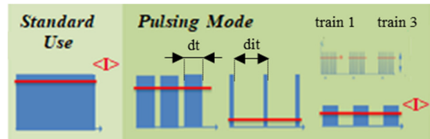
Figure 1: Examples of variable time structure with the new pulsing chopper-based system. 3 trains of bunches are represented. \langle I \rangle is the average intensity.
