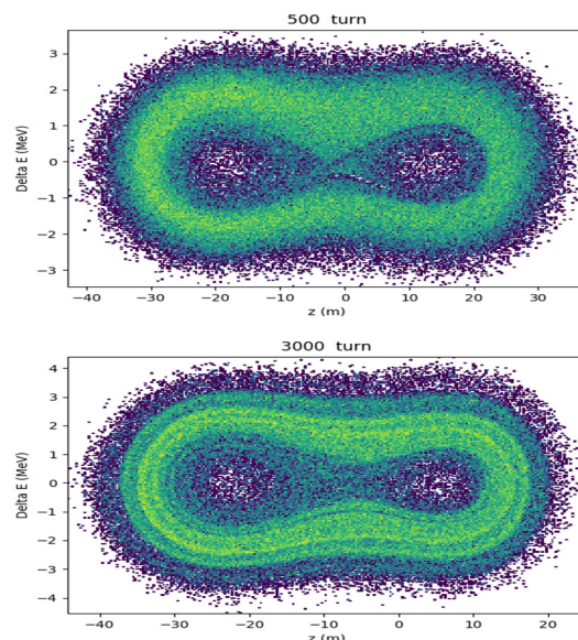
Figure 4: Longitudinal phase space of different turns at the same acceleration period.
