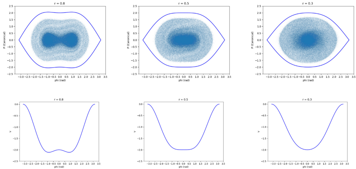
Figure 2: The longitudinal phase space and potential function with dual harmonic RF system while r equals 0.8, 0.5, 0.3 from left to right separately. The phase space density is proportional to the potential function value. The definition of coordinates can be found in reference[6].
