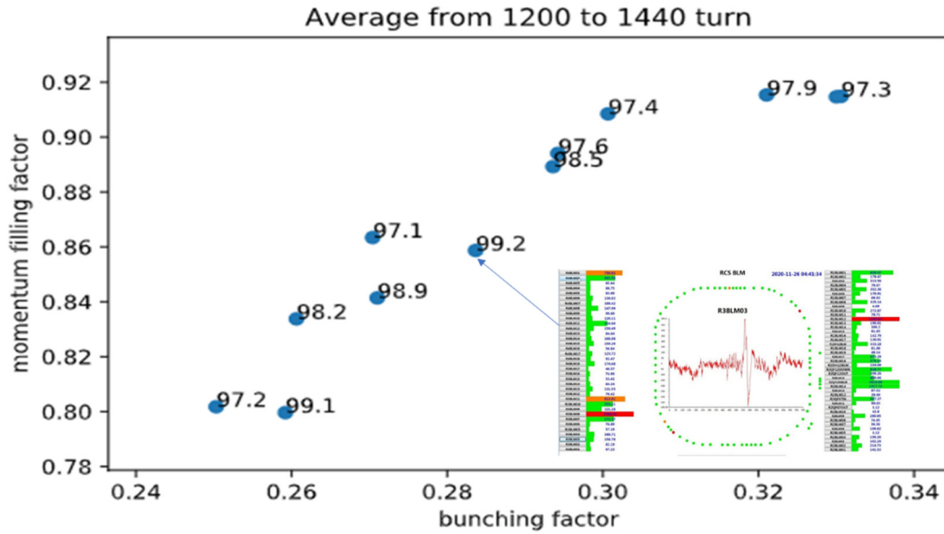
Figure 1: Comparison of RCS transmission under different longitudinal parameters. The beam loss distribution is measured by beam loss monitor, and the red bar near the arc section means large beam loss occur.
