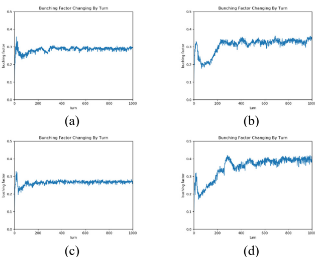
Figure 3: The simulation results of bunching factor by using PyORBIT with J-PARC's parameter at 181MeV [7]. The pictures above are respectively: (a) r = 0.5 ; (b) r = 0.5 and -0.2\% momentum offset; (c) r = 0.8 ; (d) r = 0.8 and -0.2\% momentum offset.
