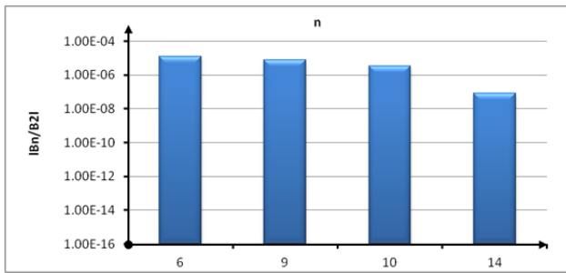
Figure 7: Absolute normalized multipoles' error at radius of 10mm.
