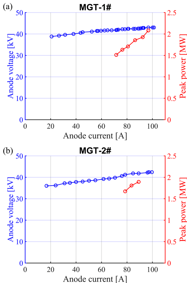
Figure 4: Performance characteristics of (a) “MGT-1#” and (b) “MGT-2#”.
