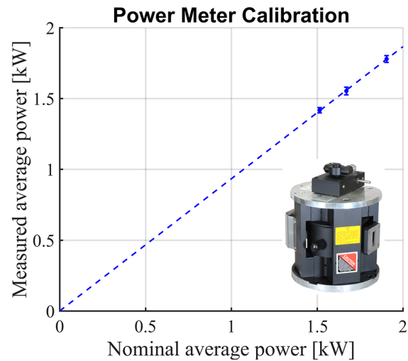
Figure 3: Calibration of water-loading calorimeter type power meter by the L3Harris magnetron [5].
