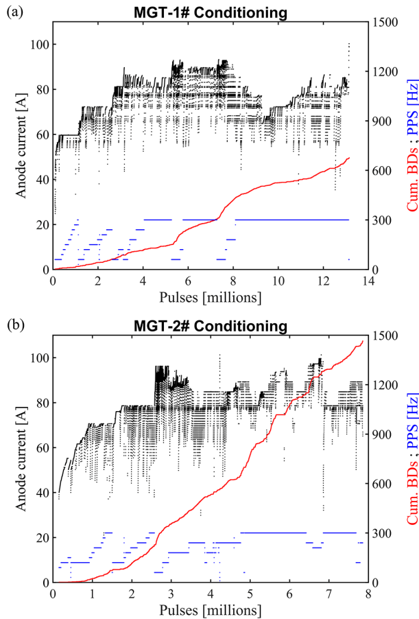
Figure 2: Conditioning histories of (a) “MGT-1#” and (b) “MGT-2#”.
