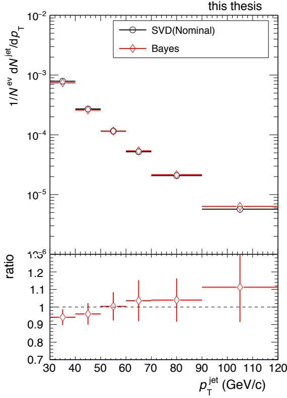
Fig 5.3: Unfolded spectra for different unfolding method selections(top), and their deviation from nominal selection(bottom), in 0-10% centrality class.
