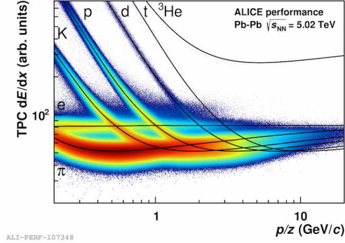
Fig 2.11: TPC dE/dx as a function of momentum with superimposed Bethe-Bloch lines for various particle species, measured in Pb-Pb collisions at \sqrt{s_{NN}} = 5.02 TeV. [33]
