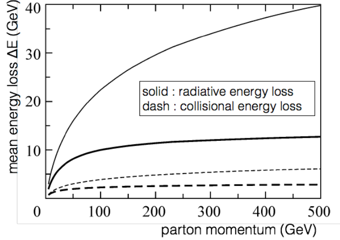
Fig 1.9: Light quark radiative and collisional energy loss for \sqrt{s_{\text{NN}}} = 5.5 TeV conditions for L=5\text{fm} . The thick curves correspond to the running \alpha_s and thin curves to \alpha_s = 0.5 , utilise the T-dependent Debye mass from the lattice calculations. [26]
