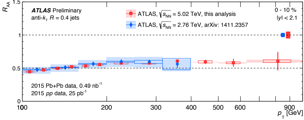
Fig 6.5: Comparison of nuclear modification factor of jets with R = 0.4 measured by ATLAS between \sqrt{s_{\text{NN}}} = 2.76 TeV and \sqrt{s_{\text{NN}}} = 5.02 TeV. [58]
