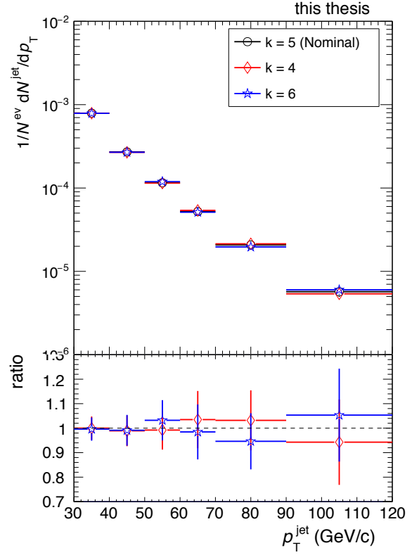
Fig 5.4: Unfolded spectra for different regularisation parameter selections(top), and their deviations from nominal selection(bottom), in 0-10% centrality class.
