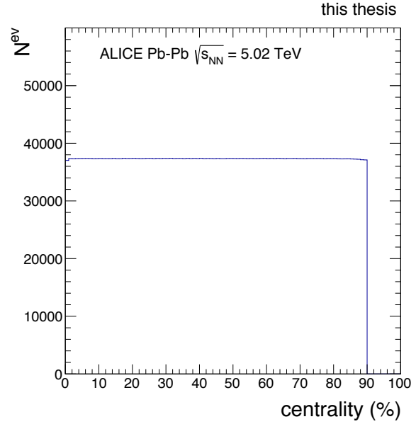
Fig 4.2: Event centrality distribution calculated with the V0M (= V0A + V0C) estimator.
