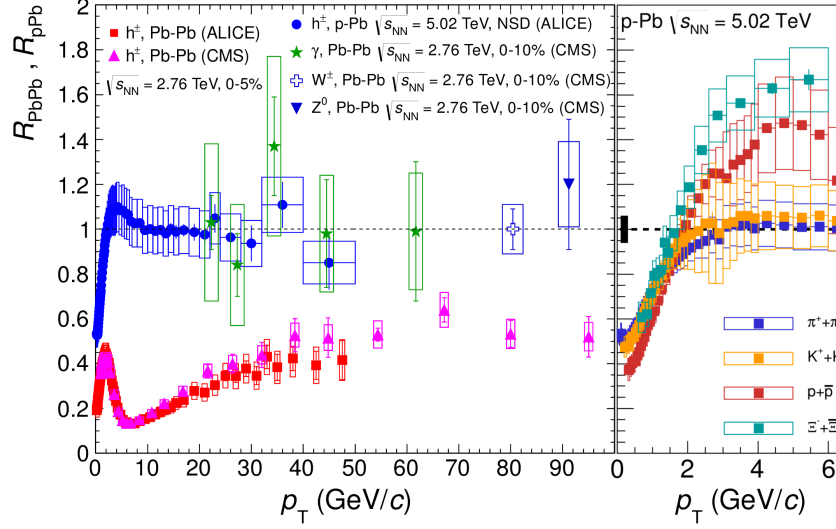
Fig 1.11: (left) Single particle nuclear modification factor R_{AA} (for Pb-Pb collisions at \sqrt{s_{NN}} = 2.76 TeV) and R_{pA} (for p-Pb collisions at \sqrt{s_{NN}} = 5.02 TeV) of particles at LHC energies. (right) for four particle species. [27]
