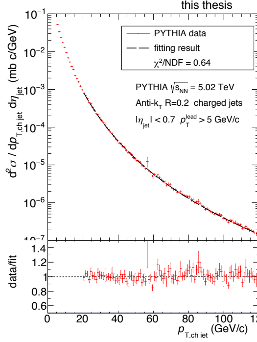
Fig 6.6: (top) PYTHIA Charged jet spectrum given by PYTHIA. The black line is Tsallis fitting result. (bottom) The ratio of data to fitting function.
