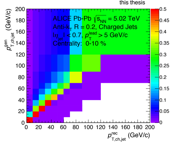
Fig 4.22: Response Matrix on detector effects in 0-10% centrality class.
