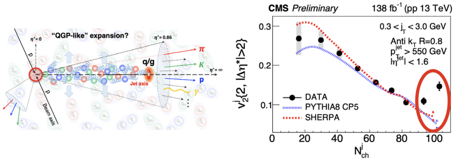
Figure 6. Left: sketch of jet reference frame as used for the elliptic flow coefficient measurement of CMS as a function of jet charged-particle multiplicity. Right: elliptic flow coefficient as a function of jet charged-particle multiplicity density compared to predictions from PYTHIA 8 and SHERPA. Figures from [10].
