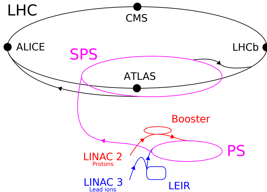
Figure 2.3.: Schematic of the CERN accelerator chain from the initial particle sources and LINear ACcelerators (LINACs) to the LHC. Adapted from Reference [11], other experiments using these accelerators not shown.
