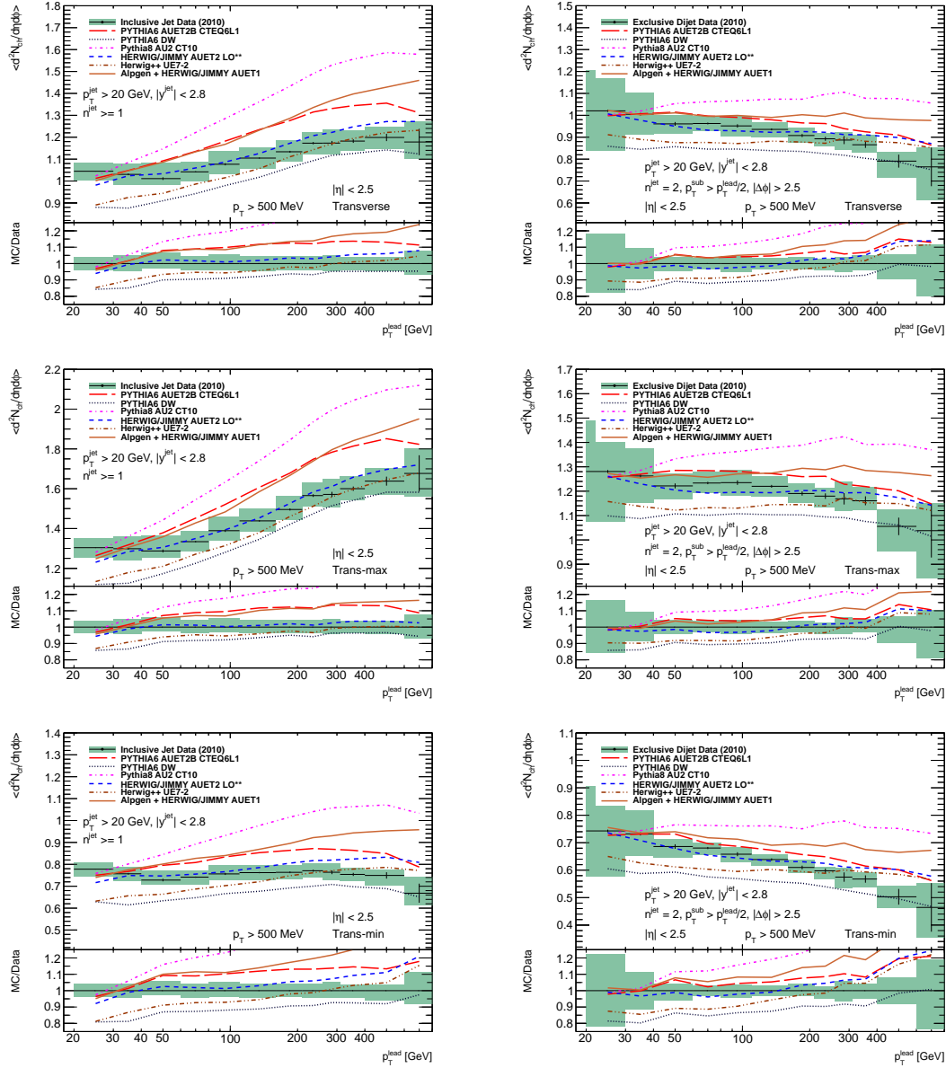
Figure 8.2.: Charged particle N_{ch} vs. p_T^{lead} profiles, shown from top to bottom for the transverse, trans-max and trans-min regions. Inclusive leading jet and exclusive di-jet selections in the left and right columns respectively.
