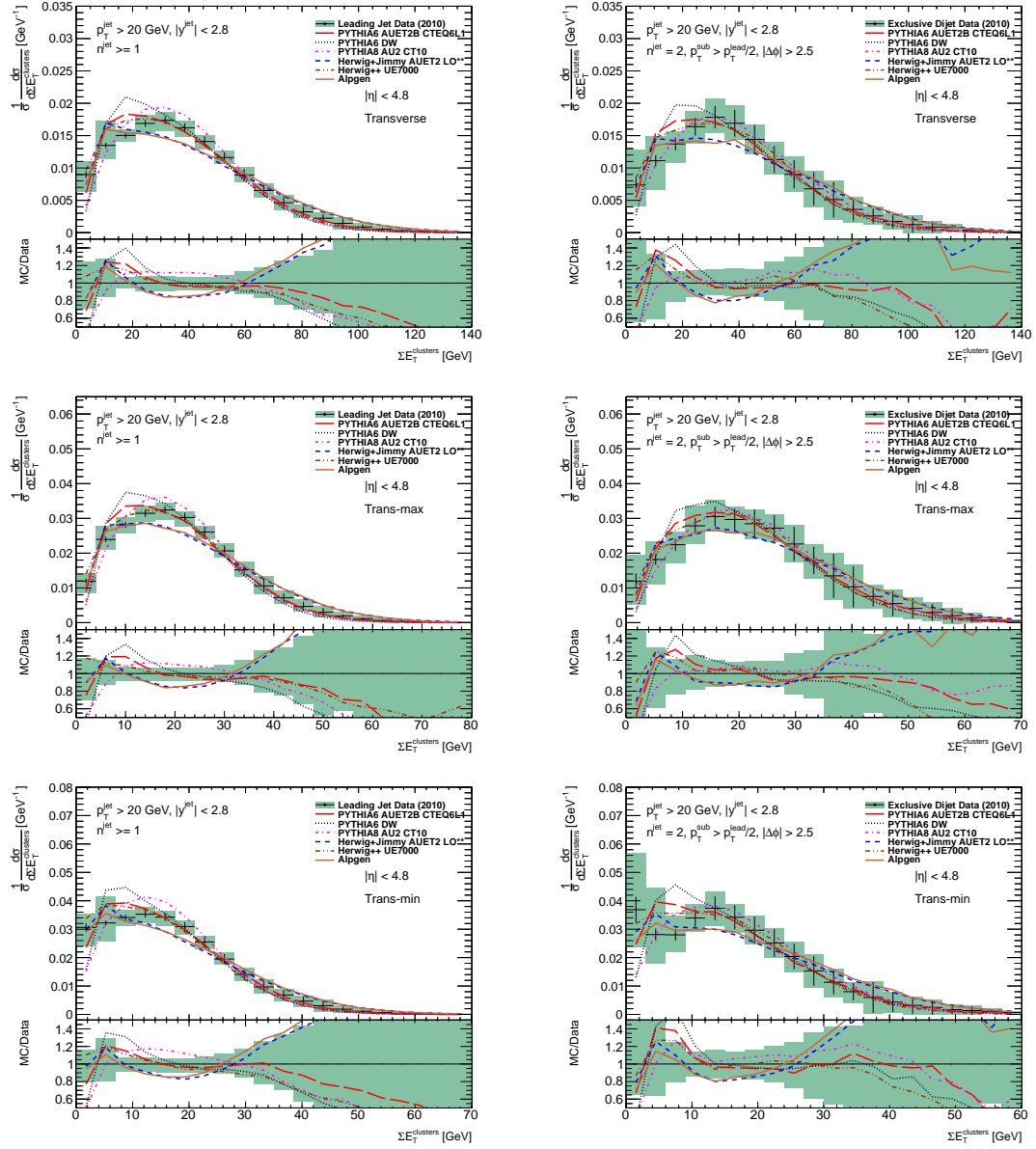
Figure D.3.: Topocluster \Sigma E_T distributions ( |\eta| < 4.8 ) shown from top to bottom for the transverse, trans-max and trans-min regions. Inclusive leading jet and exclusive di-jet selections in the left and right columns respectively.
