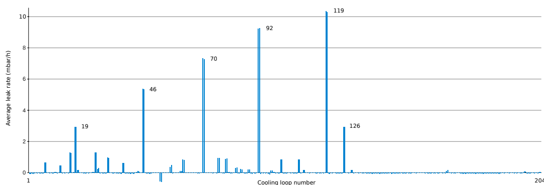
Figure 3.7.: Plot showing the average leak rates of all cooling loops for the leak-down test from January 7 th – 13 th 2010. Loops with leak rates over 2 mbar h -1 are labelled.
