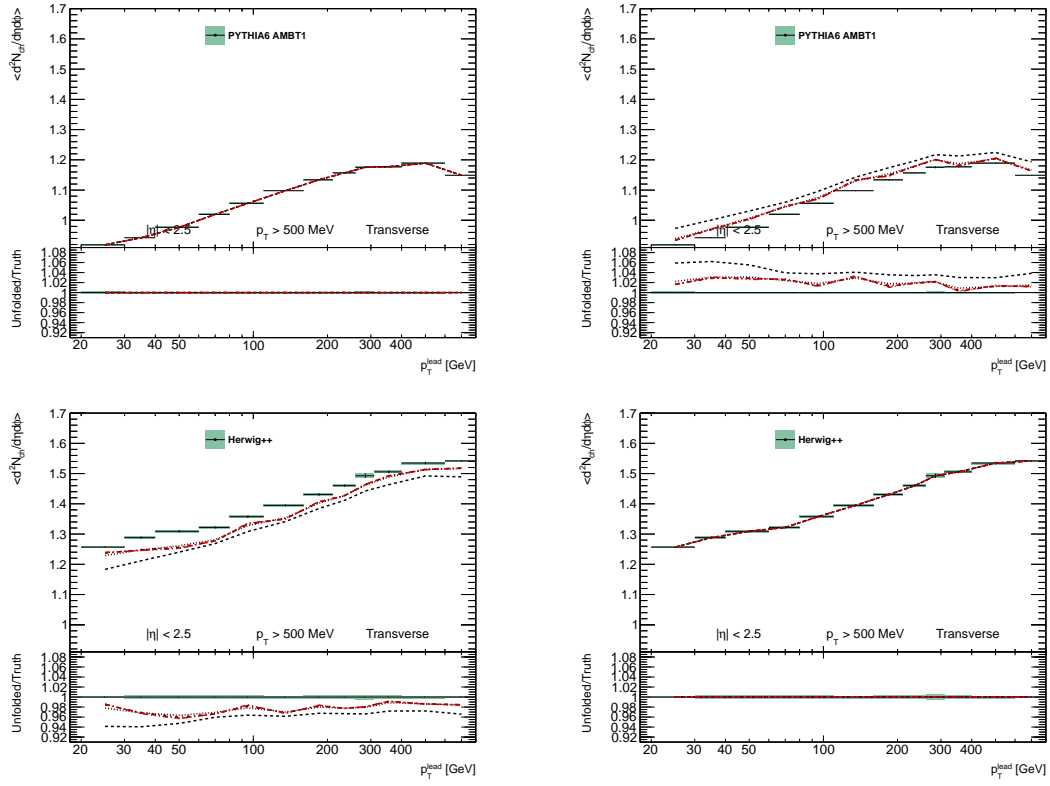
Figure A.3.: Results shown for the transverse region – leading jet selection – charged particle N_{ch} vs. p_T^{lead} . In the top row, the AMBT1 reco distribution is unfolded using prior and smearing matrix from AMBT1 (left) and Herwig++ (right). In the bottom row, the Herwig++ reco distribution is unfolded using prior and smearing matrix from AMBT1 (left) and Herwig++ (right).
