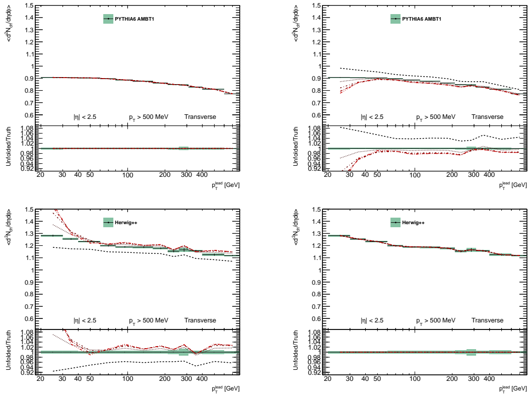
Figure A.4.: Results shown for the transverse region – exclusive di-jet selection – charged particle N_{ch} vs. p_T^{lead} . In the top row, the AMBT1 reco distribution is unfolded using prior and smearing matrix from AMBT1 (left) and Herwig++ (right). In the bottom row, the Herwig++ reco distribution is unfolded using prior and smearing matrix from AMBT1 (left) and Herwig++ (right).
