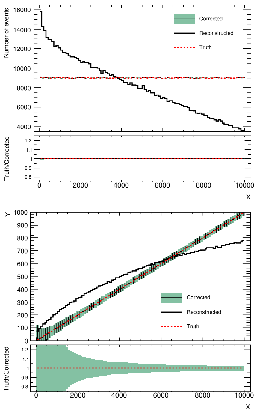
Figure 7.3.: Events have uniformly distributed values for the observables X and Y , and X = 10Y . A Gaussian smearing is applied, then Imagirol used to correct for this and recover the true variable distributions. In the upper plot, the points showing the corrected X distribution fall exactly on the horizontal line of the true distribution. In the lower plot, the points showing the corrected X vs Y distribution fall exactly on the line X = 10Y of the true distribution. Both plots show perfect closure, despite each reconstructed distribution differing substantially from the truth. Corrected distributions show statistical errors as narrow bars, with a shaded background showing the statistical and systematic errors combined in quadrature.
