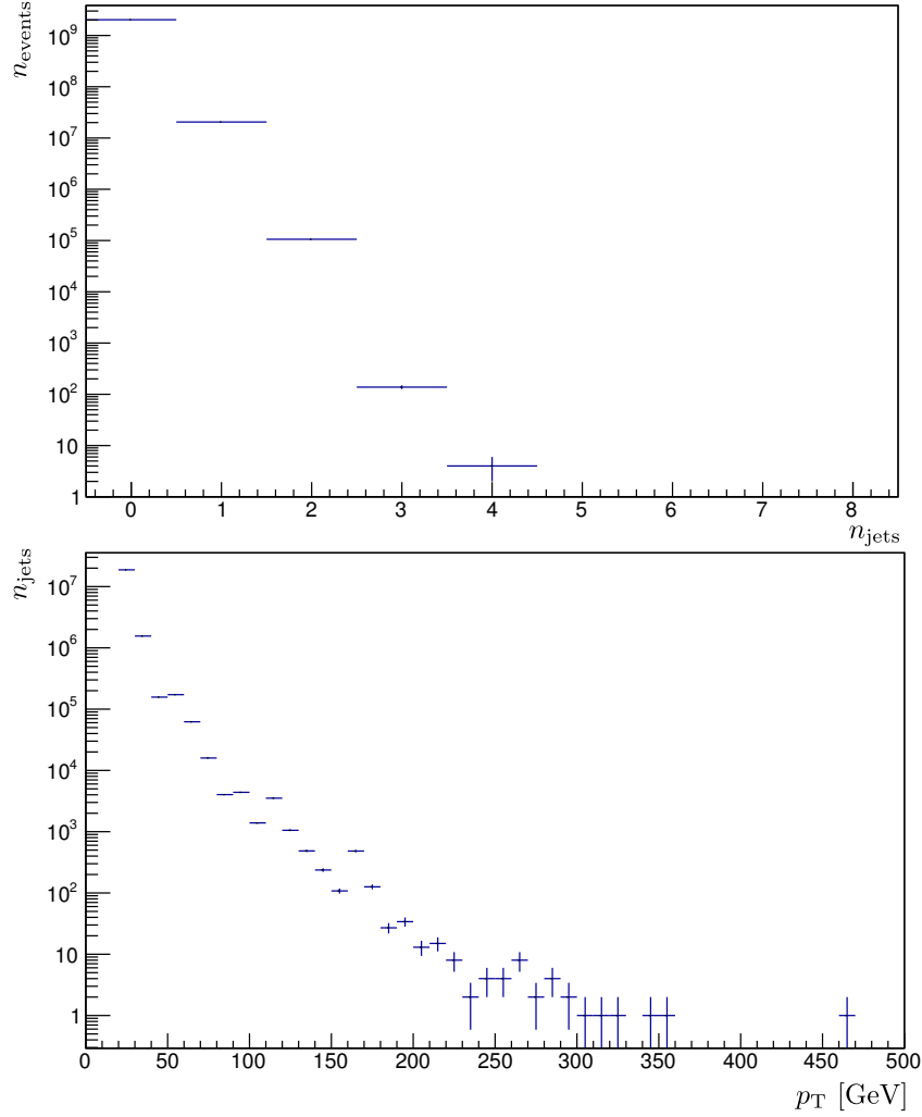
Figure 8.11.: The multiplicity (top) and p_T (bottom) distributions of jets found in the transverse region of events passing the inclusive leading jet selection. These results are presented at detector level.
