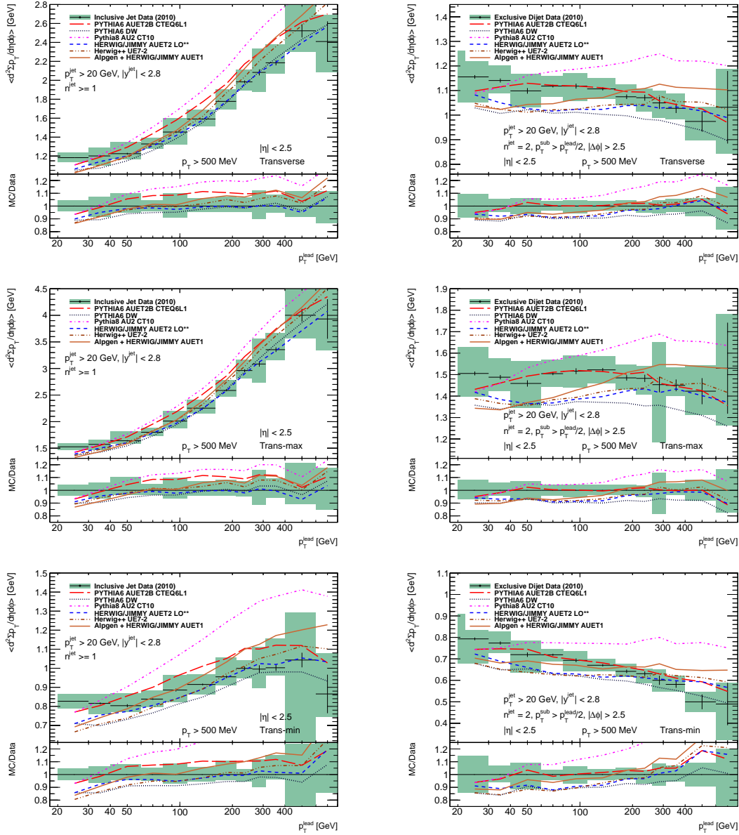
Figure 8.1: Charged particle \sum p_T vs. p_T^{\text{lead}} profiles, shown from top to bottom for the transverse, trans-max and trans-min regions. Inclusive leading jet and exclusive di-jet selections in the left and right columns respectively.
