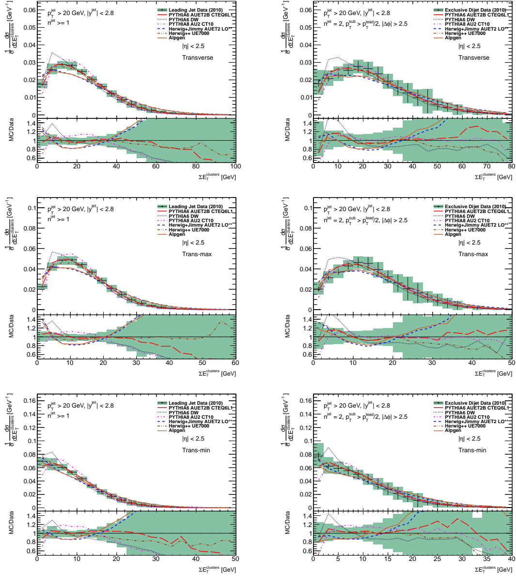
Figure D.4.: Topocluster \Sigma E_T distributions ( |\eta| < 2.5 ) shown from top to bottom for the transverse, trans-max and trans-min regions. Inclusive leading jet and exclusive di-jet selections in the left and right columns respectively.
