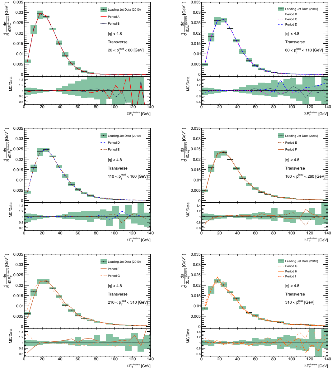
Figure B.4.: Comparison of the topocluster \Sigma E_T distributions ( |\eta| < 4.8 ) in the transverse region for the data periods and p_T^{\text{lead}} ranges indicated.
