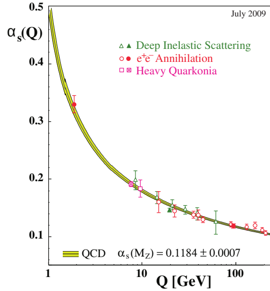
Figure 4.4.: The variation of \alpha_s with Q , also called the running coupling of QCD [54]. Different data-point styles indicate the source of the result. Full symbols are results based on N3LO QCD, open circles are based on NNLO, open triangles and squares on NLO QCD. The cross-filled square is a computational result based on lattice QCD.
