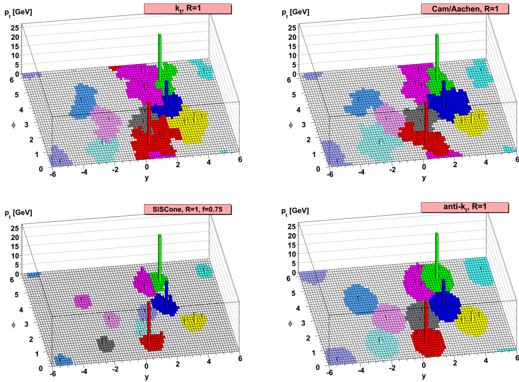
Figure 4.8.: Example of clustering particles in the same event to form jets using different algorithms [70]. Note the additional parameter f in the SIScone result, which indicates the fraction of momentum that must be shared by two overlapping cones for them to be merged into a single jet candidate.
