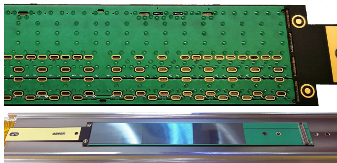
Figure 38. Example of an assembled MFT ladder. Upper picture: back side of the FPC with the glue spots on which the sensor are glued. Bottom picture: front view of assembled ladder.
