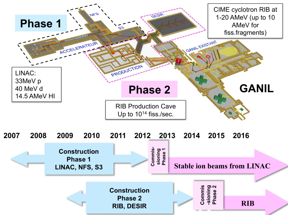
Fig. 1. Upper part: the layout of the SPIRAL2 facility indicating two construction phases. Phase 1 with the LINAC, NFS and S3 experimental halls; Phase 2: RIB production building and DESIR experimental hall. The timeline corresponding to the two construction phases is presented in the lower part of the figure.
