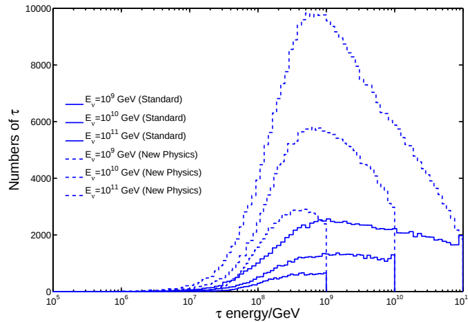
Fig. 1. The tau-lepton energy spectra resulting from Earth-skimming tau neutrinos with different initial energies and a 20 km medium length. The solid lines are results obtained from standard neutrino–nucleon scattering cross section while the dashed lines are those obtained from enhanced scattering cross section, \sigma_{\text{NEW}} = 10 \sigma_{\text{SM}} . Each curve is generated with 10^6 incoming neutrino events.
