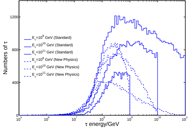
Fig. 2. The same as Fig. 1 except that the medium length is 100 km.
