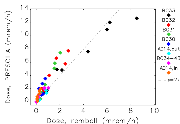
Figure 3: Comparison of neutron dose for two instruments at 1-m, Scenario 2, with varying beam current (6 GeV).
