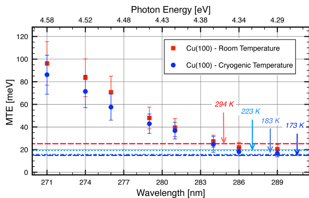
Figure 2: MTE values for a single crystal Copper (100) cathode at two different temperatures. The lower energy limit at different temperatures is shown by dotted lines.
