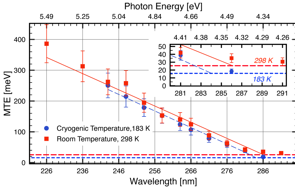
Figure 1: MTE values for a copper (100) single-crystal cathode at two different temperatures. The MTE lower threshold defined by k_B T is shown by the red and blue horizontal dotted lines for T = 298 and 183 K respectively, with the inset showing the detail close to the photoemission threshold.
