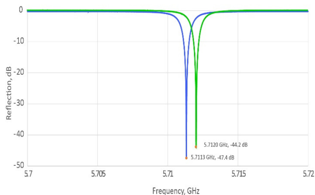
Figure 2: The results of the cold-test measurements for the two \beta=0.5 cavities. The green line is for the copper cavity, and the blue line is for the copper-silver cavity.
