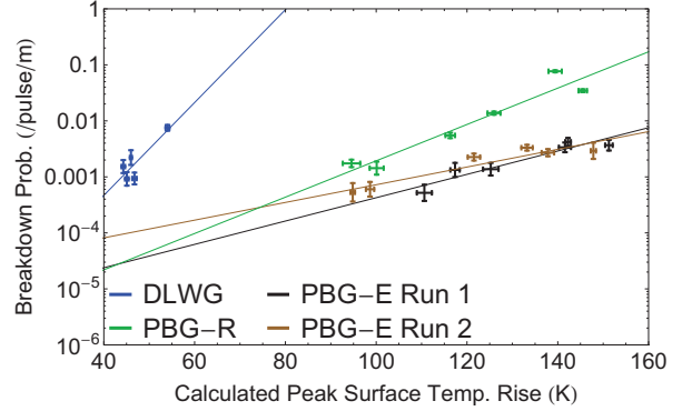
Figure 4: Breakdown probability per pulse per meter of structure vs. calculated peak pulsed heating for the PBG-R, PBG-E, and a conventional disc-loaded waveguide structure with the same iris geometry (DLWG) at a pulse length of 150 ns.
