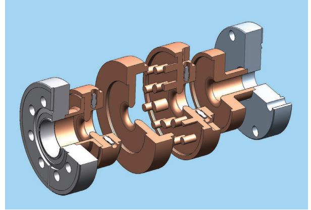
Figure 1: Expanded three-quarter view of solid model of elliptical-rod PBG structure, showing two coupling cells and central PBG cell. Power is coupled in from the left.
