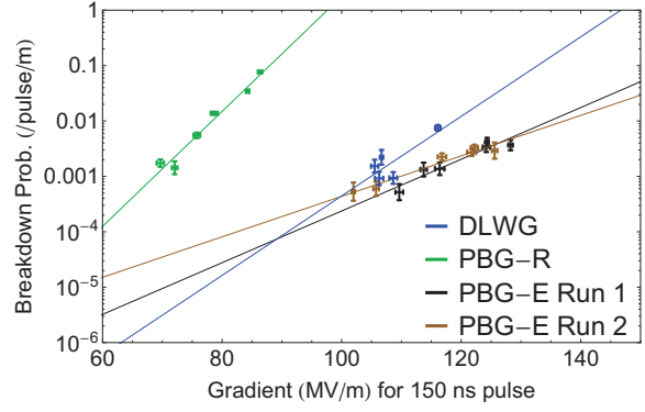
Figure 3: Breakdown probability per pulse per meter of structure vs. gradient at 150 ns pulse length for the PBG-R, PBG-E, and an undamped conventional disc-loaded waveguide structure with the same iris geometry (DLWG). The two data sets for the PBG-E represent the beginning and end of testing.
