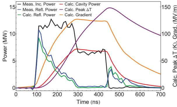
Figure 2: Sample traces from the peak power meter for a 150 ns pulse at a gradient of 126 MV/m. The incident and reflected power measured by the peak power meter are shown in black and blue respectively. The calculated reflected power and power coupled into the structure are shown in green and red respectively. The calculated gradient is shown in orange, and the calculated peak surface temperature rise is shown in purple.
