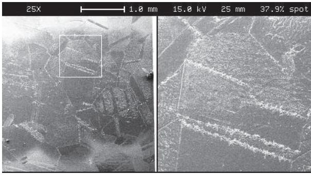
Figure 5: Detail micrograph of the high-field side of the inner rod of the PBG-E, showing grain boundaries even at the highest-field region.
