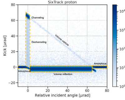
Fig. 1. Simulated proton angular kick distribution as a function of relative angle between incoming particles and crystal orientation with SixTrack after a single pass through the crystal. Protons at 6.5 TeV are considered.
