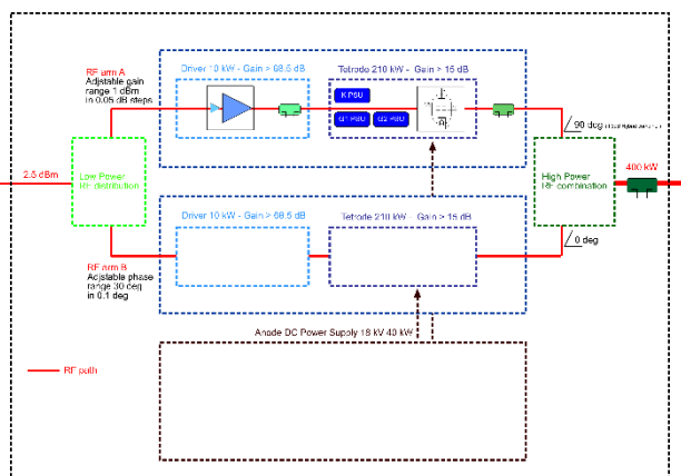
Figure 1: RF amplification chain layout.
