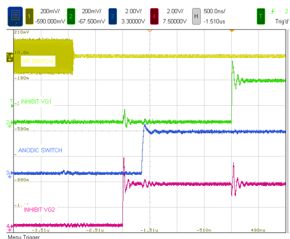
Figure 4: Fast interlock signals.
