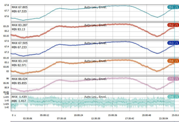
Figure 6: RF power data in dBm for all the amplification stages recorded over 24 hours. The RF power drift is due to the cooling water temperature poor stabilization.
