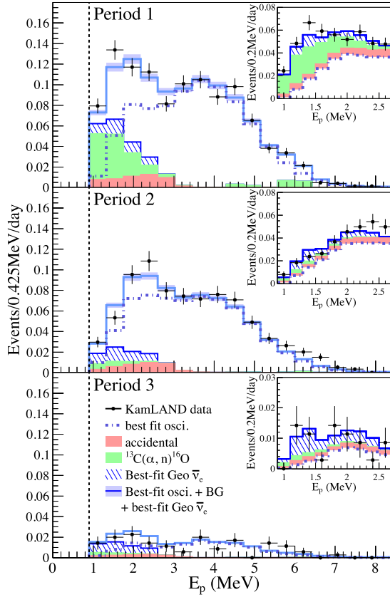
Fig. 4. Prompt energy spectrum of \bar{\nu}_e -candidate events for each data taking period (see Fig. 3), the inset shows the prompt spectrum with a finer binning for low-energy events. KamLAND suffered from a large radioactive background in the first period of data taking. This was significantly reduced after a purification campaign (Period 2). Period 3 is after the installation of an inner-balloon for the KamLAND-Zen experiment in September 2011. It coincides with a low reactor neutrino flux period following the Fukushima reactor accident. Figure adapted from [8].
