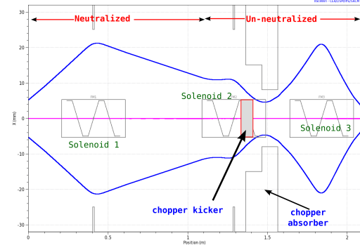
Figure 2: Beam envelope in the LEBT
