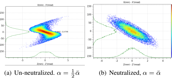
Figure 3: Horizontal phase space at the RFQ input.
