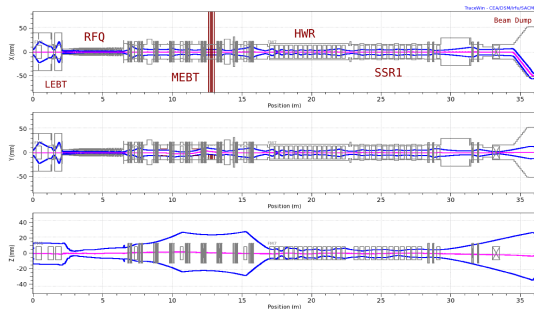
Figure 1: PXIE end-to-end 3\sigma beam envelopes. Top: (x, x') , Middle: (y, y') , Bottom: (z, z') . The MEBT is shown operating in transmission mode. The beam sweep magnet is shown steering horizontally over the dump area.
