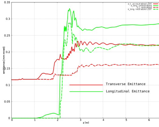
Figure 4: Emittance evolution through the RFQ. Solid: LEBT with un-neutralized section. Dashed: Fully neutralized LEBT.
