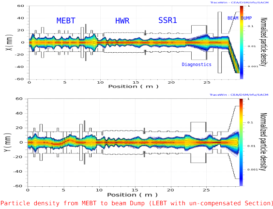
Figure 5: Particle density from the MEBT to the beam dump area.
