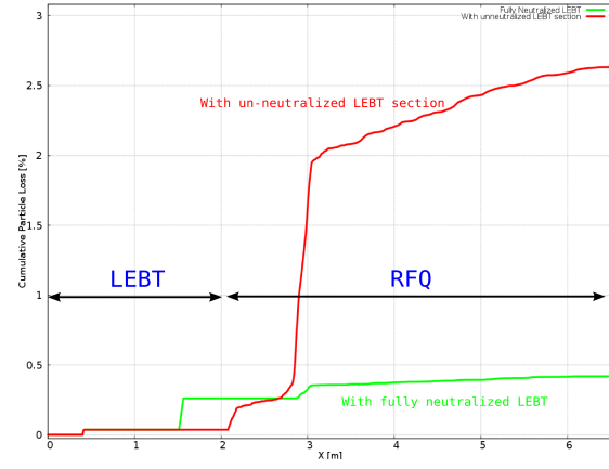
Figure 6: Cumulative particle losses from the source to the RFQ output.
