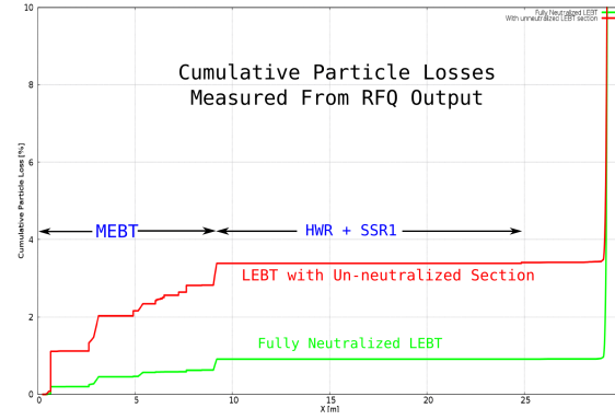
Figure 7: Cumulative particle losses from the MEBT to the beam dump.
