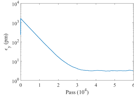
Figure 8: Vertical emittance obtained after a single energy modulation for the different turns.
