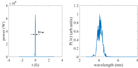
Figure 7: Power distribution (left) and spectrum (right) of the radiation pulse.
