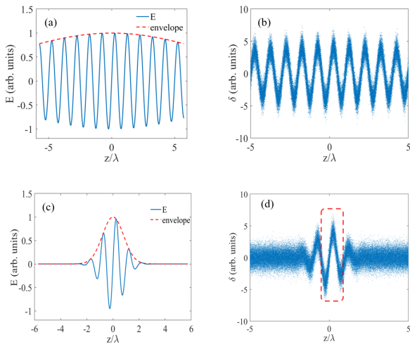
Figure 2: Electric field and the envelope of the many-cycle (a) and few-cycle (c) laser. Longitudinal phase space of the electron beam after the many-cycle (b) and few-cycle (d) laser modulation.
