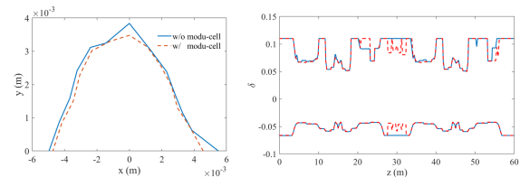
Figure 5: Dynamic aperture (left) and the momentum aperture (right) for the case with and without modu-cell.
