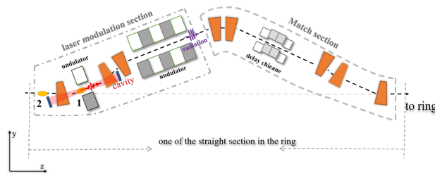
Figure 1: Layout of the proposed scheme.
