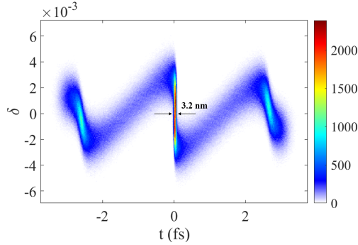
Figure 6: Longitudinal phase-space of the electron beam before enters the radiator.
