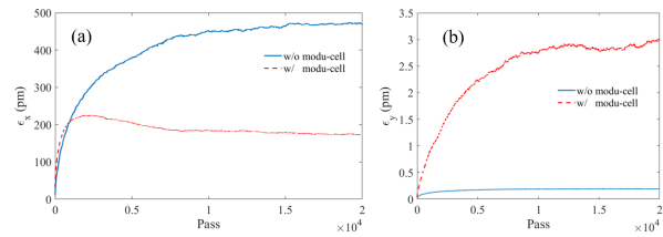
Figure 4: Horizontal (a) and vertical (b) emittance varying with different turns for the case of with and without the modu-cell.
