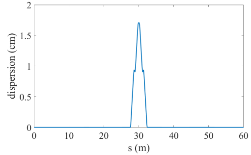
Figure 3: Vertical dispersion of the modu-cell.
