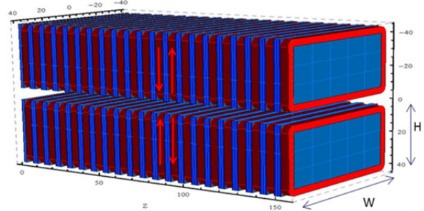
Figure 1: The radia model for the planar SCU.
