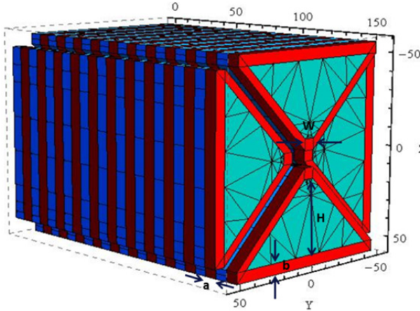
Figure 3: The Radia model for the helical SCU.
