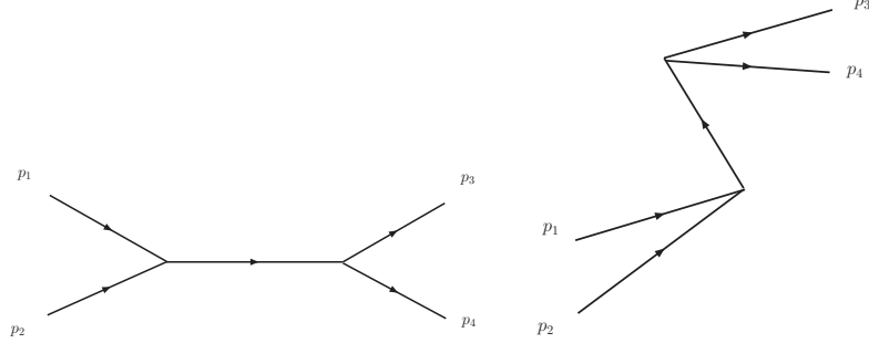
Fig. 1. The 2 \rightarrow 2 process in the \phi^3 theory, decomposed into two different time ordered diagrams. Left: diagram which is left in the infinite momentum frame. Right: vacuum graph which vanishes in this frame.
