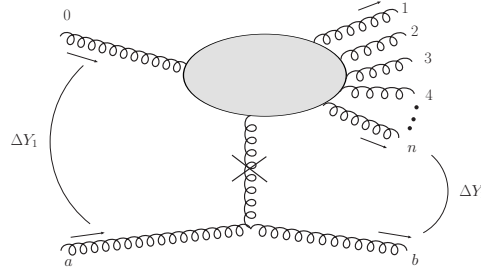
Fig. 2. The 2 \rightarrow n+1 on-shell gluon amplitude in the high energy limit. The gluon 0 dissociates into the gluon cascade (indicated by a blob) which interacts via high energy gluon (with a cross) with the gluon a \rightarrow b . The large rapidity difference \Delta Y_1 \sim \Delta Y_2 between the light-front cascade and the lower gluon is taken. The arrows indicate the momentum flow: the gluons 0, a are incoming and 1, \dots, n, b are outgoing. All the gluons have + helicity and it is conserved.
