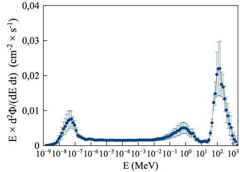
Figure 6: Neutron spectrum measured at Testa Grigia in July 2022 (multiplied by energy).
