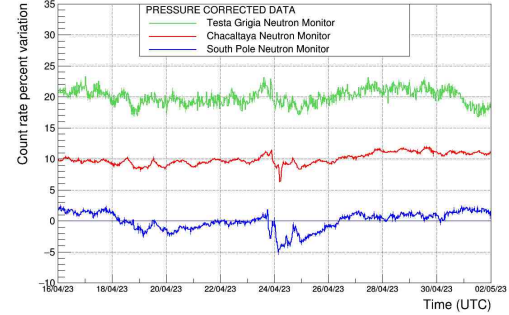
Figure 8: Percent variations of the Chacaltaya neutron monitor counting rates, compared with the data of the South Pole and Testa Grigia neutron monitor during 16 days around the G4 solar storm on 23 April 2023.
