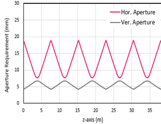
Figure 6: Half-aperture requirement for the SPS-II booster synchrotron.
