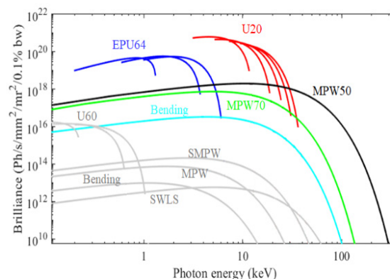
Figure 1: Brilliance of synchrotron light radiated as a function of photon energy from the existing 1.2 GeV machine (grey) and SPS-II (color).
