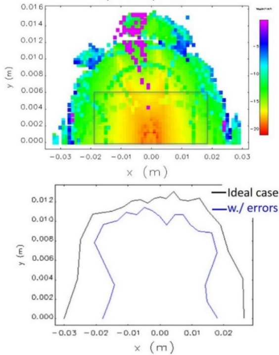
Figure 5: Booster dynamic aperture at the nominal working point (top) and dynamic aperture including the misalignment and lattice imperfections (bottom).
