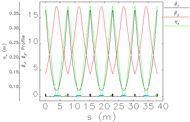
Figure 4: Optical functions for one symmetric lattice, (Maximum horizontal betatron functions = 16.3 m, maximum vertical betatron function = 17.1 m, and maximum dispersion function = 0.377 m).
