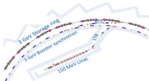
Figure 2: Layout design of SPS-II source with a 150 MeV linac and a 3 GeV booster sharing in the same tunnel as storage ring.
