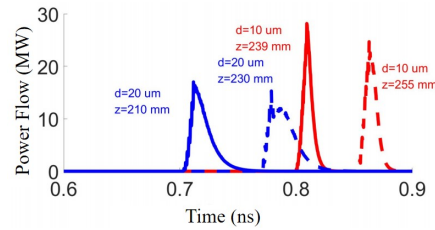
Figure 6: Power flow vs time at the cross sections where the maximum power and pulse energy are achieved respectively.
