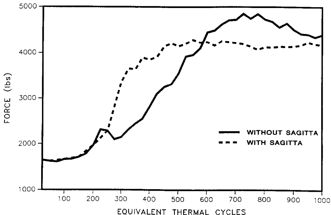
Fig. 5. D0004 Full Length Slide Tests
