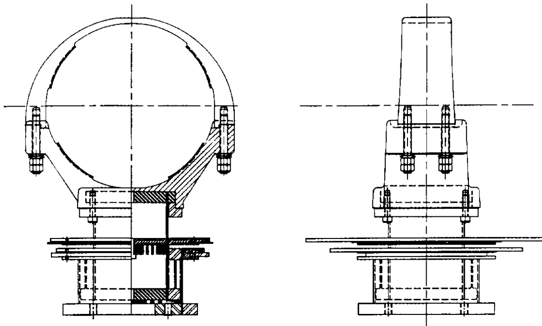
Fig. 4. Design B Slide Connection Casting
