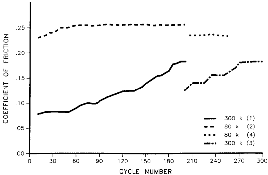
Fig. 2. Design A Friction vs. Equivalent Thermal Cycles
