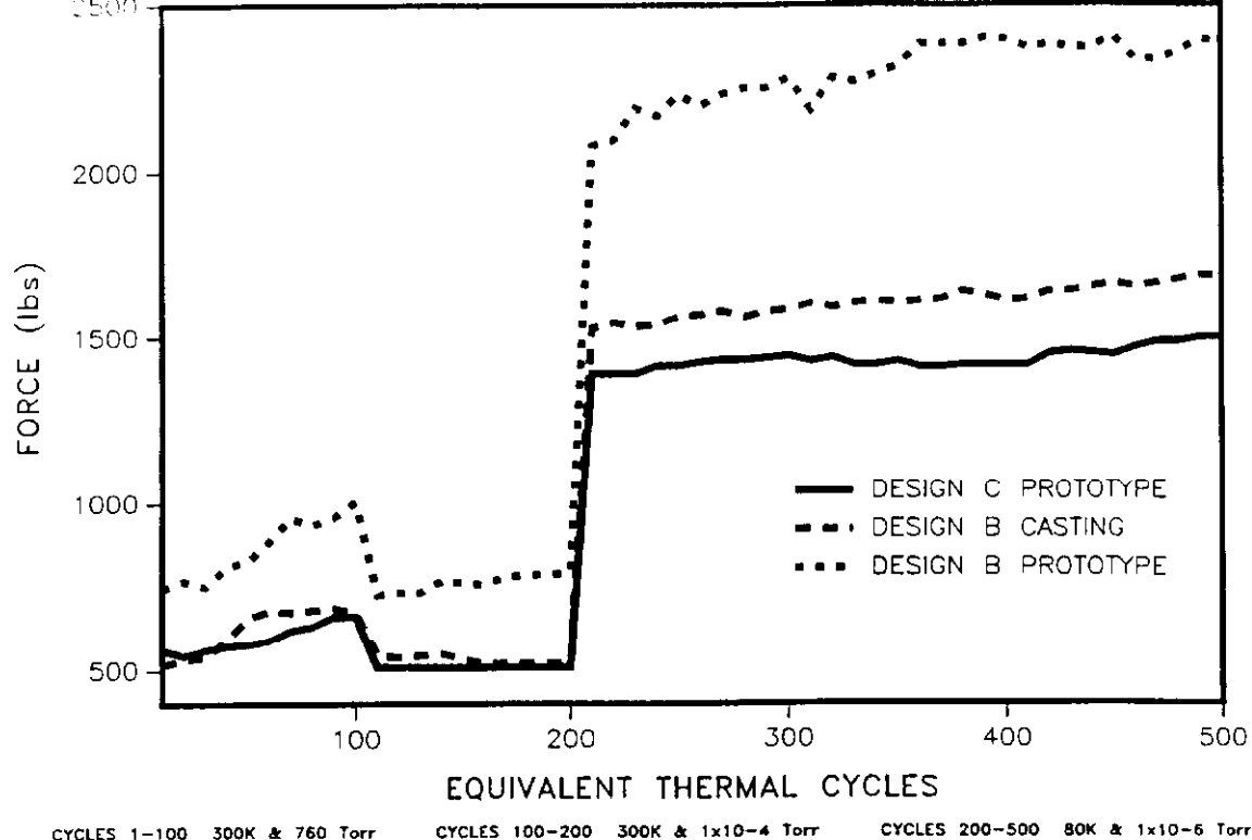
Fig. 6. Cold Slide Test Comparison
