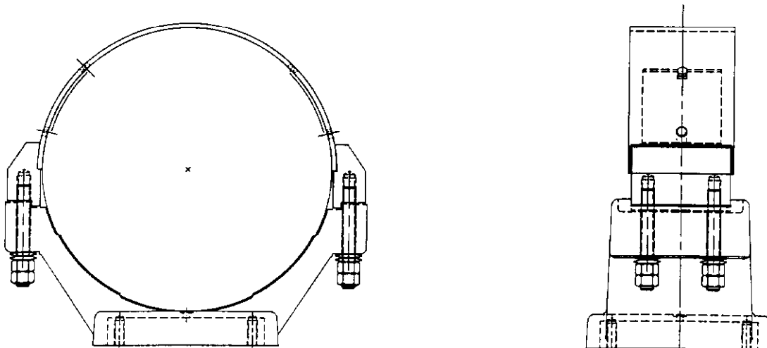
Fig. 7. Design C Prototype Slide Connection
