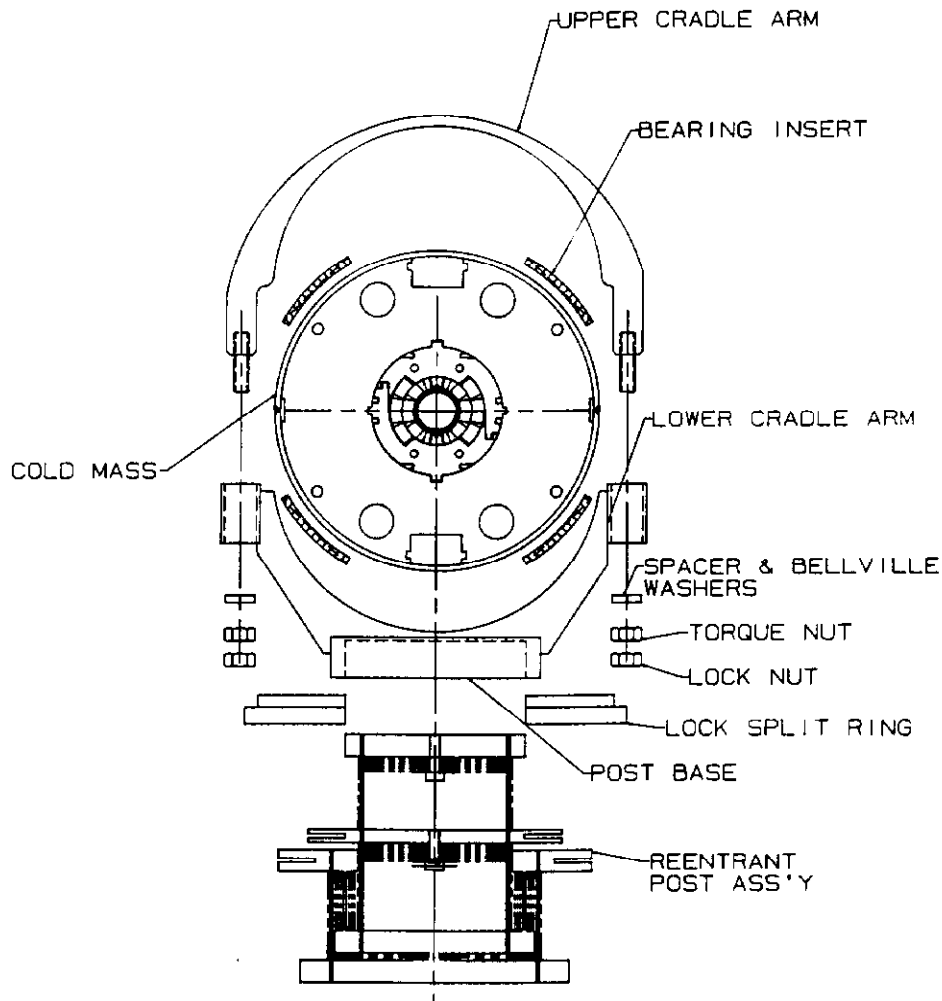
Fig. 3. Prototype Design B Slide Connection
