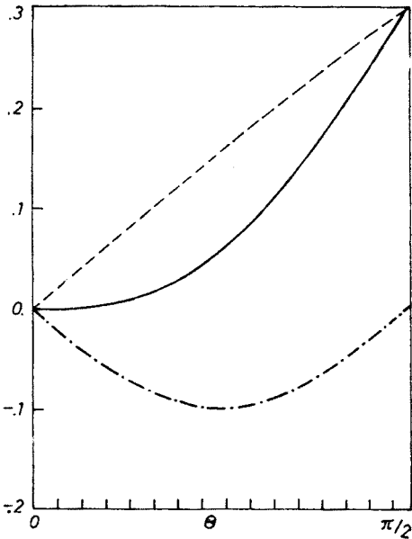
Fig. 2. Second moment of the baryon number radial distribution in the vacuum: M_2^{vac}(\theta) (solid line, M_{K=0}^{(2)} (dashed line) and M_{K>0}^{(2)} (dashed-dotted line)
