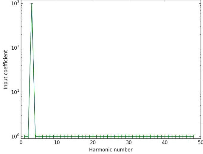
Figure C.1: Harmonic spectrum used as input for verification of Bootstrap method. Values for all functions are 1 except the 3rd function, for which the value is equal 1000.
