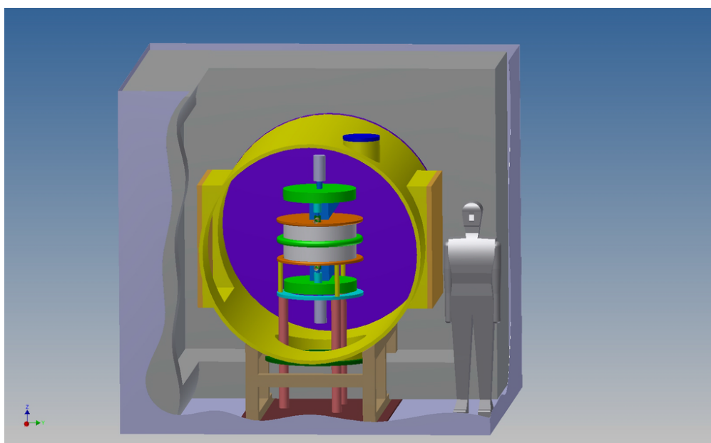
Figure 2.12: Preliminary design of n2EDM experiment apparatus. Visible are two precession chambers – designed to perform the Ramsey method of oscillatory fields with the field parallel and anti-parallel at the same time. They are positioned inside a cylindrical vacuum vessel inside a multi-layer magnetically shielded room.
