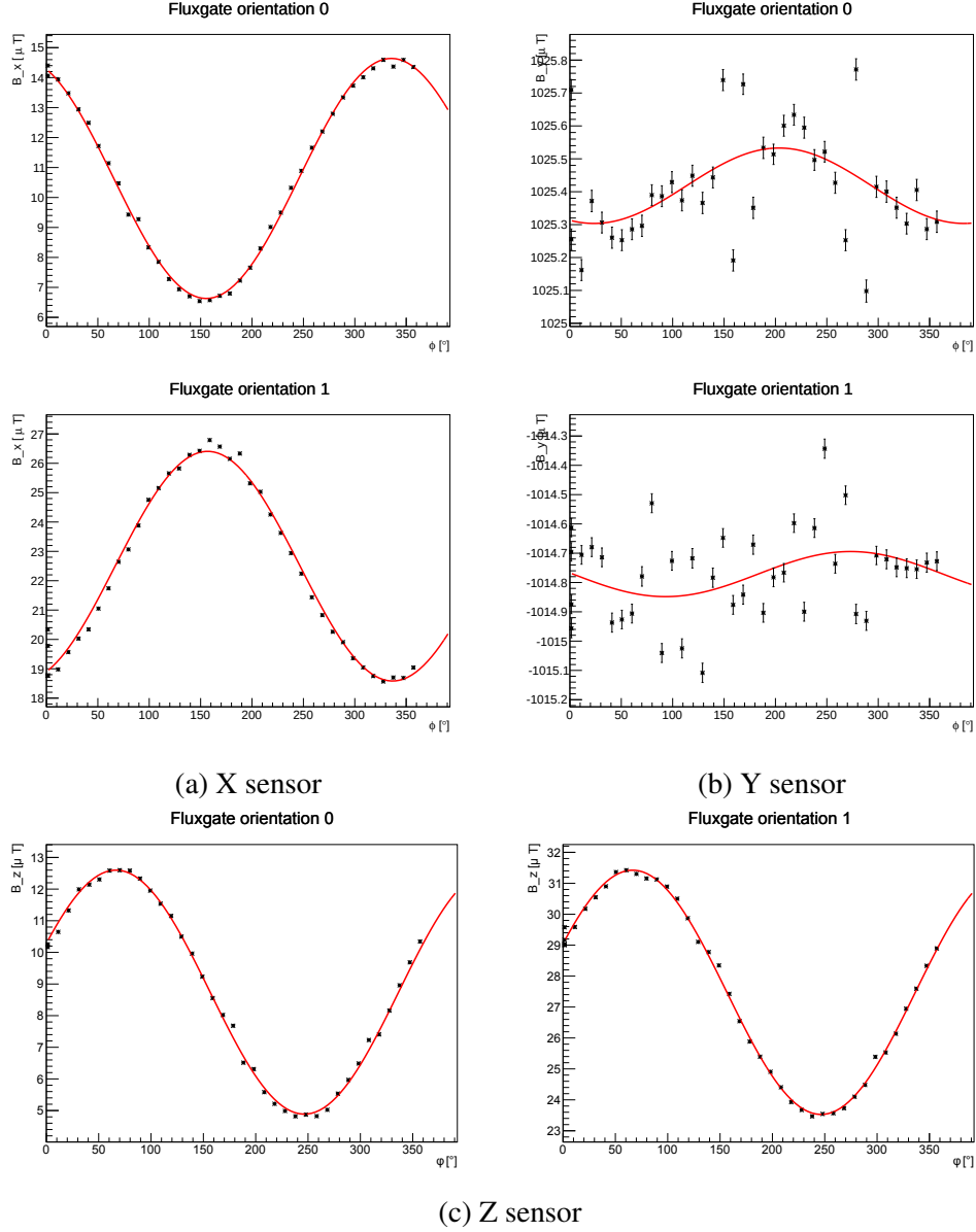
Figure 6.3: The magnetic field measured during calibration runs as a function of angle \phi . Orientation 0 corresponds to the X sensor in the \hat{\phi} direction, orientation 1 is rotated by \pi around the \hat{r} direction. This measurements are not corrected for any imperfections. Solid lines correspond to the result of the FFT fitting (for details see text).
