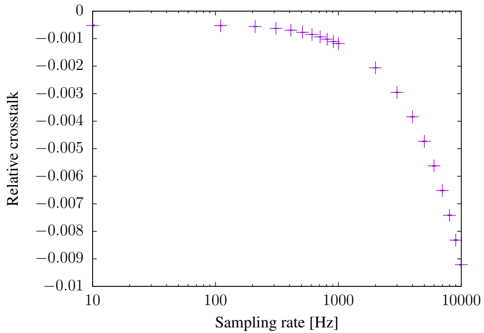
Figure 4.13: Relative crosstalk as a function of sampling rate for readout of magnetic field.
