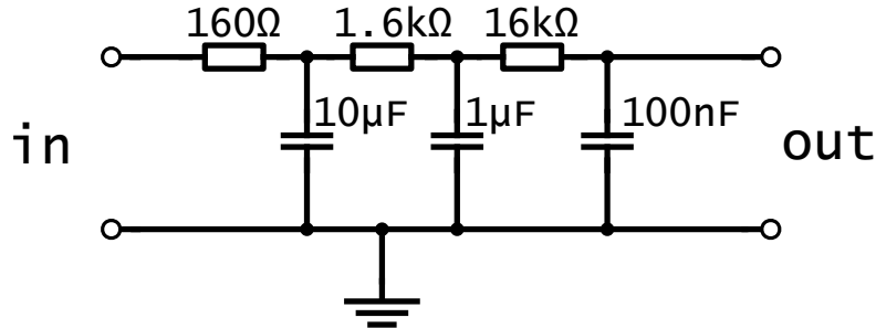
Figure 4.9: Scheme of RC filter
