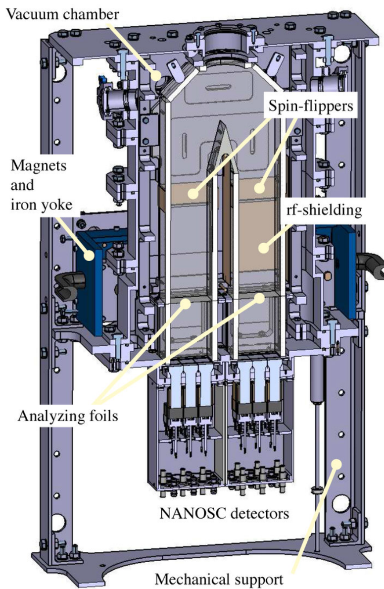
Figure 2.4: Scheme of the U-shaped Simultaneous Spin Analyser detector system
