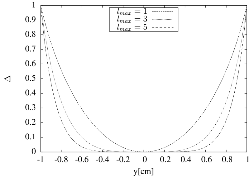
Figure 4.32: Relative difference between the analytical \vec{B} and the one calculated with VSH for a single current loop in the function of the position on the axis x = 0, z = 0 ( \Delta = \left| \vec{B}_{exact} - \vec{B}_{approx} \right| / \left| \vec{B}_{exact} \right| )
