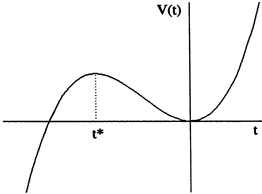
Figure 3.1: The tachyon potential in bosonic string theory.
