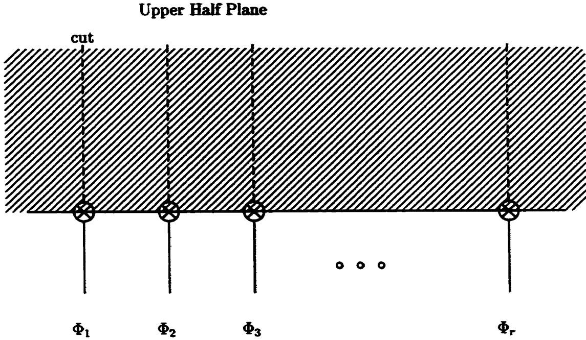
Figure 4.1: An r -point amplitude with vertex operators that carry winding numbers. It requires r cuts on the worldsheet.
