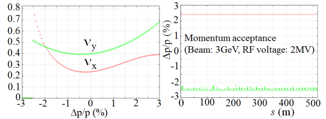
Figure 4: Fractional betatron tunes vs the momentum deviation and the corresponding momentum acceptance of TPS-2 ring.
