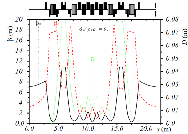
Figure 1: Lattice function of H7BA cell for TPS upgrade.
