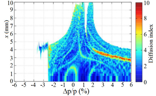
Figure 3: Diffusion index obtained from the frequency map analysis of H7BA TPS-2 upgrade lattice.
