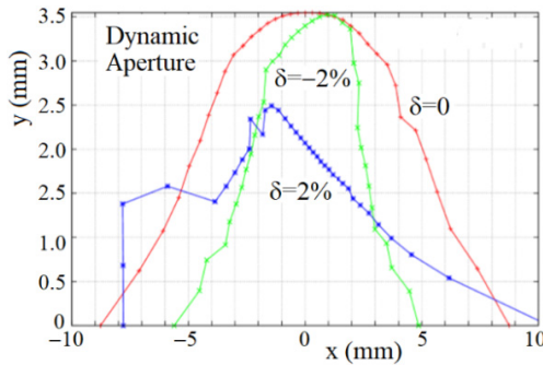
Figure 2: Dynamic aperture at the middle of straight section without multipole errors and misalignment errors.
