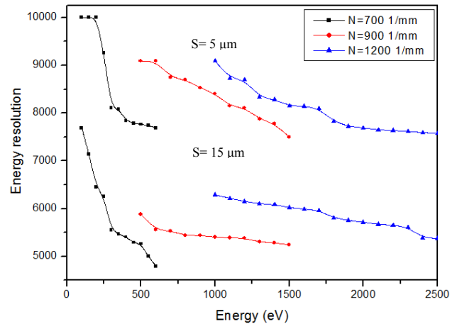
Figure 5: Monochromator resolving power at two different fixed exit slit sizes, S=5 & 15 \mu\text{m} , for three different gratings calculated by the shadow code.
