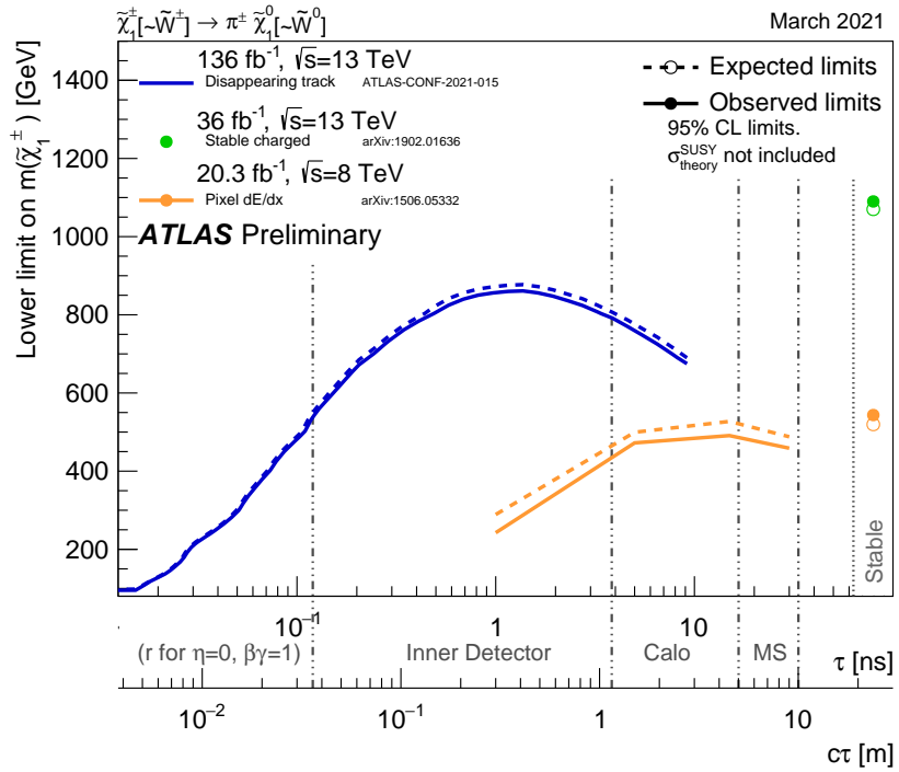
Figure 18: Constraints on the chargino mass-vs-lifetime plane for an AMSB model with \tan(\beta) = 5 and \mu > 0 . The wino-like chargino is pair-produced and decays to the wino-like neutralino and a very soft charged pion. The solid lines indicate the observed limits, while the dashed lines indicate the expected limits. The area below the curves is excluded. The analyses have sensitivity at lifetimes other than those shown, but only the limits at tested lifetimes are shown. The dots represent results for which the particle is assumed to be stable. In this context, stable means escaping the detector.
