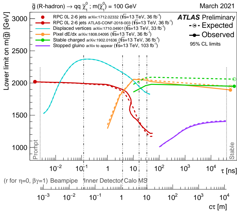
Figure 17: Constraints on the gluino mass-vs-lifetime plane for a split-supersymmetry model with the gluino R-hadron decaying into a gluon or light quarks and a neutralino with mass of 100 GeV. The solid lines indicate the observed limits, while the dashed lines indicate the expected limits. The area below the curves is excluded. For the displaced vertices result the expected and observed limits are identical. For the stopped gluino result the limit extends to larger lifetimes (not quoted here, see reference). The analyses have sensitivity at lifetimes other than those shown, but only the limits at tested lifetimes are shown. The dots represent results for which the particle is assumed to be prompt or stable. In this context, stable means escaping the detector.
