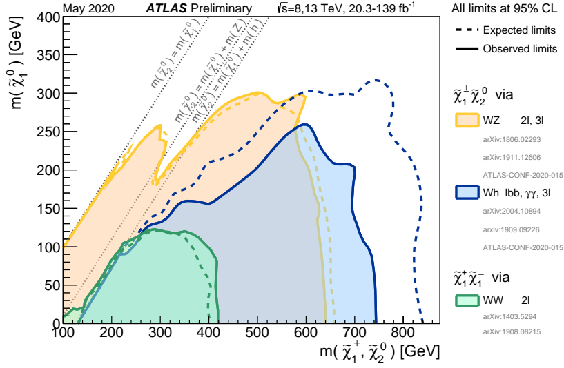
Figure 12: The 95% CL exclusion limits on \tilde{\chi}_1^\pm \tilde{\chi}_1^0 and \tilde{\chi}_1^\pm \tilde{\chi}_2^0 production with SM-boson-mediated decays, as a function of the \tilde{\chi}_1^\pm , \tilde{\chi}_2^0 and \tilde{\chi}_1^0 masses. The production cross-section is for pure wino \tilde{\chi}_1^\pm \tilde{\chi}_1^\mp and \tilde{\chi}_1^\pm \tilde{\chi}_2^0 . Each individual exclusion contour represents a union of the excluded regions of one or more analyses.
