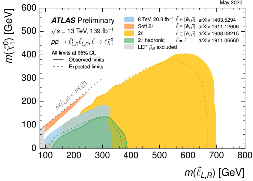
Figure 14: Exclusion limits at 95% CL based on 13 TeV data in the (slepton, lightest neutralino) mass plane for different analyses probing the direct production of sleptons with decays to lepton neutralino. The types of sleptons (flavor and coupling) included in each search is specified in the legend.
