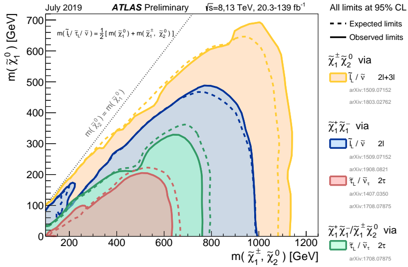
Figure 11: The 95% CL exclusion limits on \tilde{\chi}_1^\pm \tilde{\chi}_1^\mp and \tilde{\chi}_1^\pm \tilde{\chi}_2^0 production with \tilde{\ell} -mediated decays, as a function of the \tilde{\chi}_1^\pm , \tilde{\chi}_2^0 and \tilde{\chi}_1^0 masses. The production cross-section is for pure wino \tilde{\chi}_1^\pm \tilde{\chi}_1^\mp and \tilde{\chi}_1^\pm \tilde{\chi}_2^0 . Each individual exclusion contour represents a union of the excluded regions of one or more analyses.
