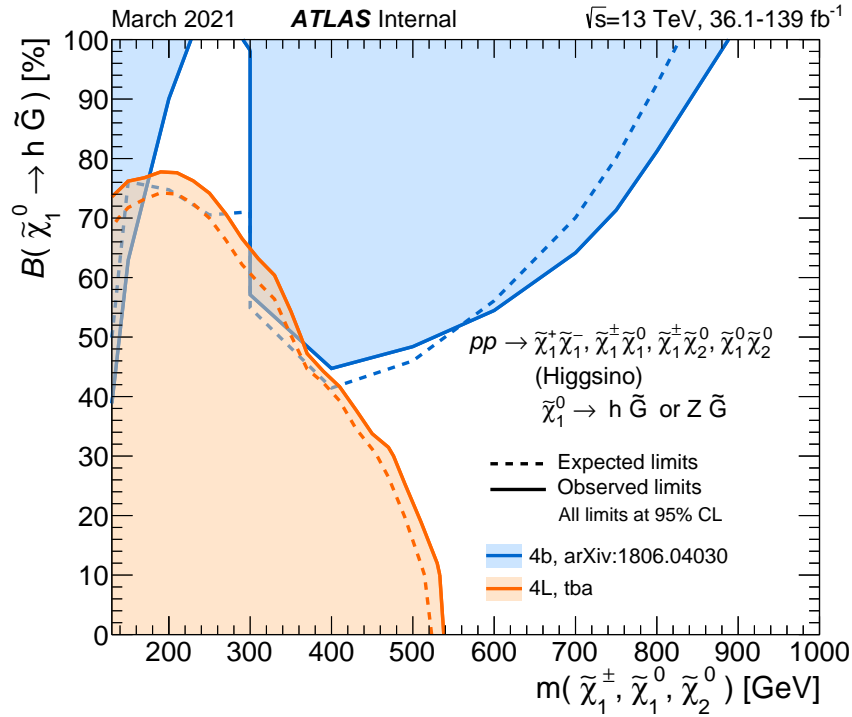
Figure 16: The 95% CL exclusion limits on a general gauge mediation model from 13 TeV data. The model assumes a pure Higgsino NLSP that promptly decays to either Z gravitino or Higgs gravitino. The limits are displayed as a function of the mass of the nearly mass-degenerate Higgsino triplet and the branching fraction of lightest Higgsino to Higgs gravitino.
