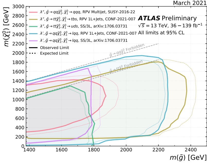
Figure 19: Exclusion limits at 95% CL based on 13 TeV data in the (gluino, lightest neutralino) mass plane for different simplified models featuring the decay of the gluino to the lightest supersymmetric particle (lightest neutralino) which in turn decays via R-parity violating couplings to Standard Model particles. For each line, the gluino decay mode is reported in the legend and it is assumed to proceed with 100% branching ratio. Some limits depend on additional assumptions, as described in the references provided in the plot.
