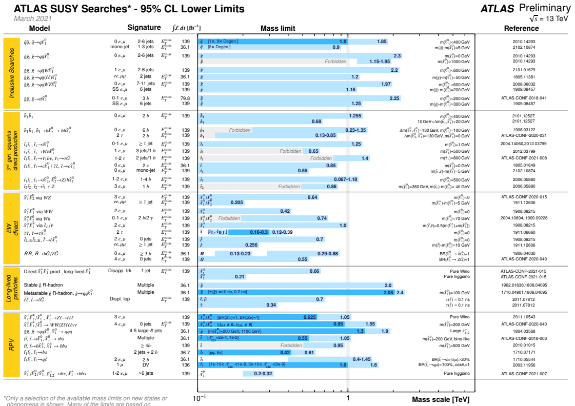
Figure 21: Mass reach of the ATLAS searches for Supersymmetry. A representative selection of the available search results is shown. Results are quoted for the nominal cross section in both a region of near-maximal mass reach and a demonstrative alternative scenario, in order to display the range in model space of search sensitivity. Some limits depend on additional assumptions on the mass of the intermediate states, as described in the references provided in the plot. In some cases these additional dependencies are indicated by darker bands showing different model parameters.
