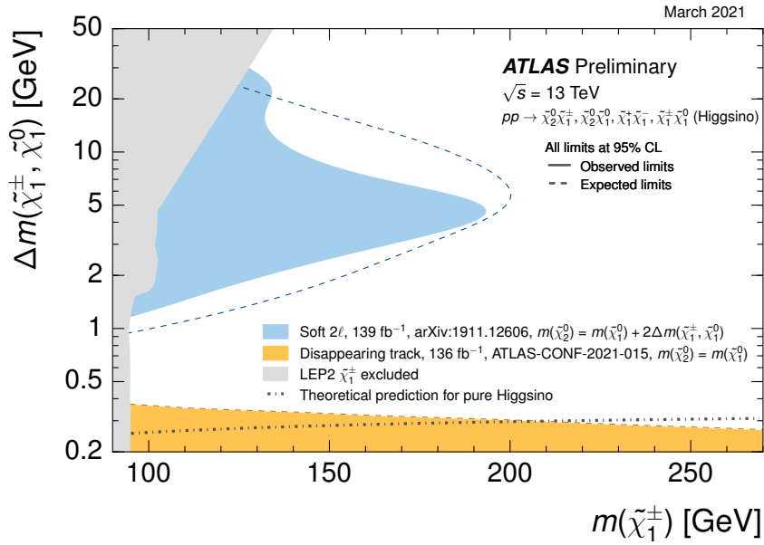
Figure 15: Exclusion limits at 95% CL for higgsino pair production \tilde{\chi}_1^+ \tilde{\chi}_1^- , \tilde{\chi}_1^\pm \tilde{\chi}_1^0 , \tilde{\chi}_1^\pm \tilde{\chi}_2^0 , and \tilde{\chi}_1^0 \tilde{\chi}_2^0 with off-shell SM-boson-mediated decays to the lightest neutralino, \tilde{\chi}_1^0 , as a function of the \tilde{\chi}_1^\pm and \tilde{\chi}_1^0 masses. The production cross-section is for pure higgsinos.
