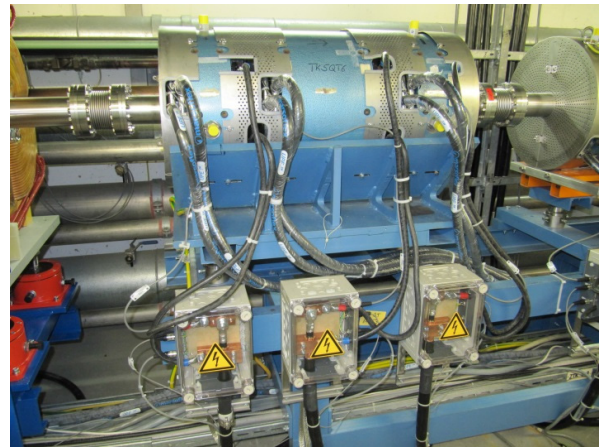
Figure 14: TK5QT6, the skew quadrupole triplet, an overhauled and modified existing GSI triplet. This is the so called “skew” triplet rotated by 45^\circ to decouple the beam.
