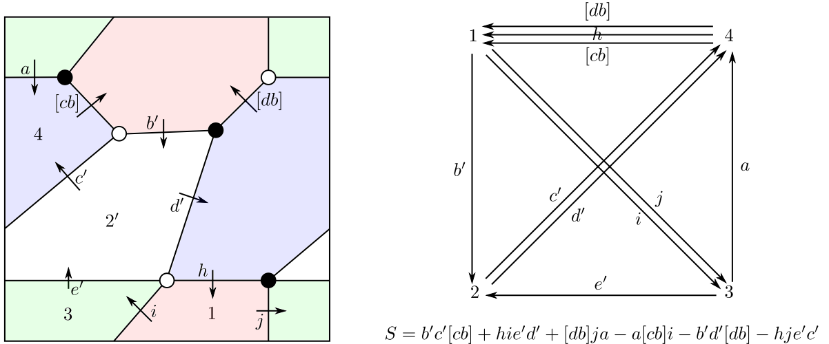
Figure 1.11: The bipartite graph, quiver and superpotential after the mutation at 2 in Figure 1.9.
