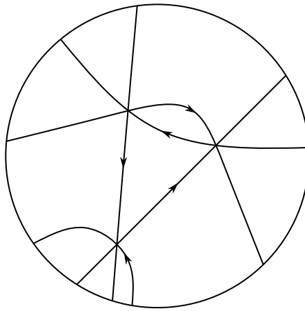
Figure 10.2: A triple diagram consisting of five strands.
