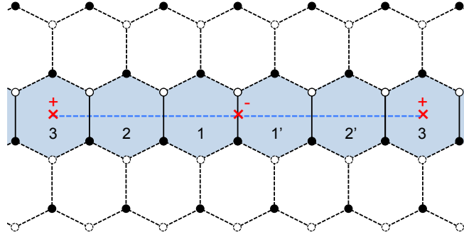
Figure 9.7: Fixed point orientifold realizing the SU(5)_1 model with SU(1)_2 flavor group and an additional SO(5)_3 factor. SO(5)_3 develops an ADS superpotential and leads to a runaway behavior.
