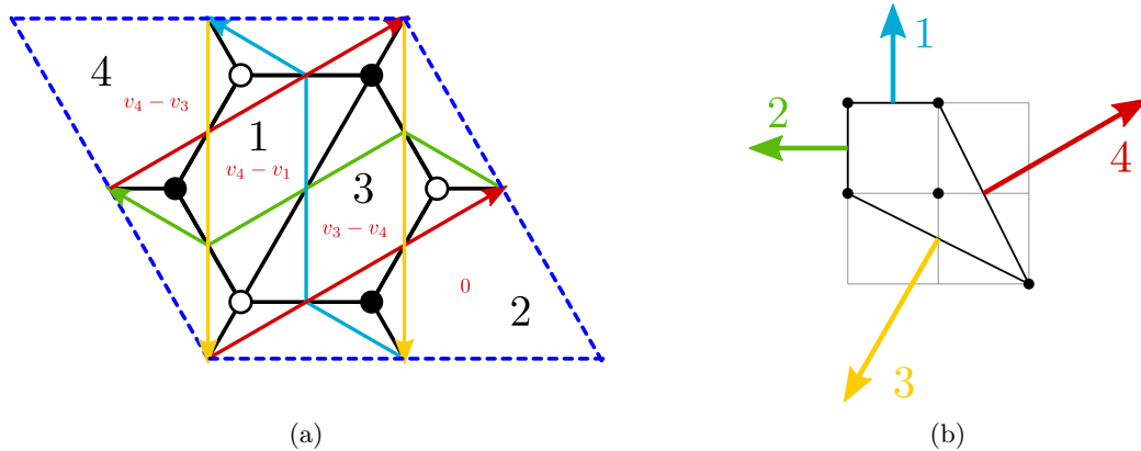
Figure 11.2: (a) Dimer diagram for dP_1 . We show the ZZPs and the rank assignments coming from them. (b) The toric/web diagram.
