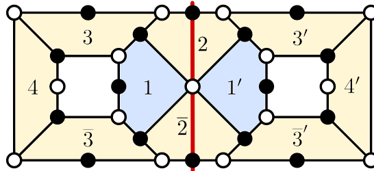
Figure 9.22: A tentative sub-dimer for a twin 3 – 2 model where the SU(3) faces share a flavor SU(1) 4 .
