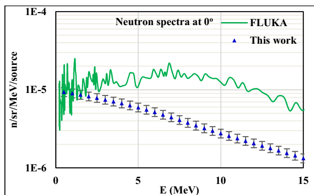
Figure 3: Unfolded spectrum of ^{208}\text{Pb} (6.25 MeV/u) + ^{\text{nat}}\text{Cu} compared to the FLUKA simulation.
