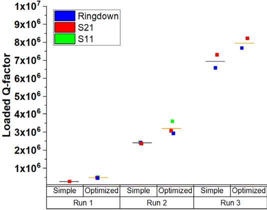
Figure 6: Comparison of measured Q-factors of optimized and non-optimized Nb resonators at 10 mK, measured by different methods in different runs at a single photon level.
