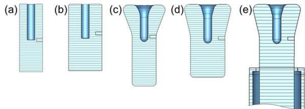
Figure 2: QWR design optimization: reference model (a), optimized straight geometry (b), optimal design not feasible with machining (c), final design optimized for machining fabrication (d) and design with RF choke (e).
