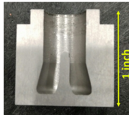
Figure 1: Section of machined niobium qubit 3D resonator with the optimized shape.
