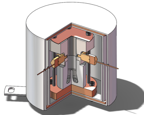
Figure 3: Full assembly with two layers of magnetic shielding, IR shield copper cap, SMA penetrations, and niobium 3D resonator.
