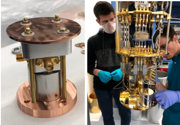
Figure 5: 3D QWR assembly (left), attached to the 10mK stage of the dilution refrigerator at the University of Chicago (right).
