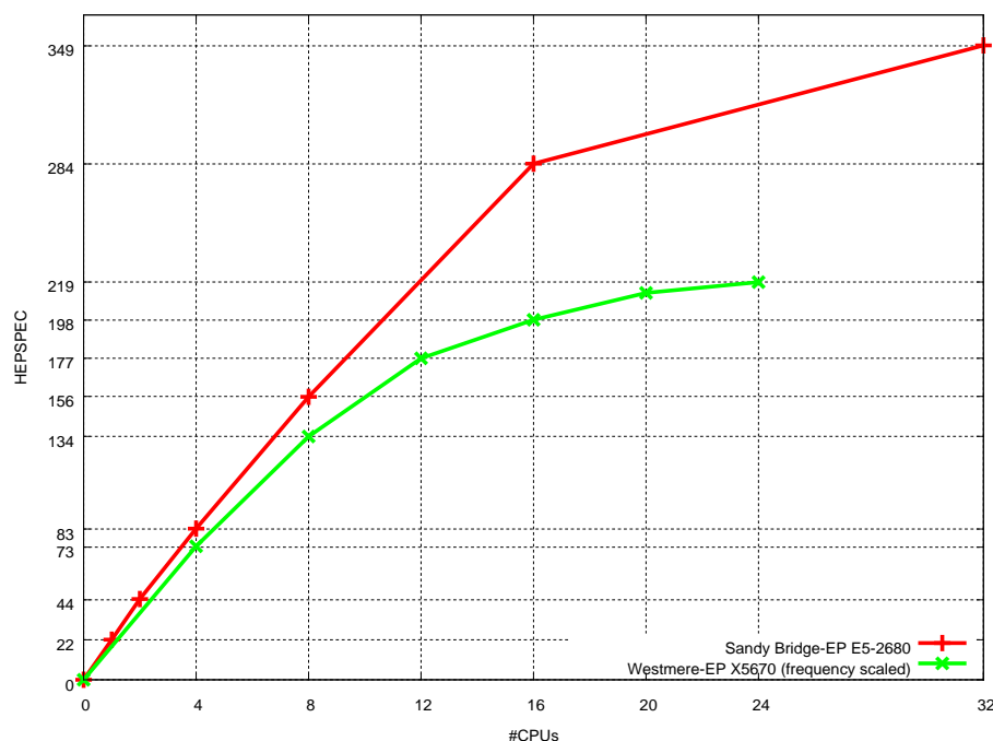
Figure 6. HEPSPEC06 performance comparison “Sandy Bridge-EP” E5-2680 vs. “Westmere-EP” X5670 (frequency scaled). Both systems have SMT on and Turbo mode disabled.
