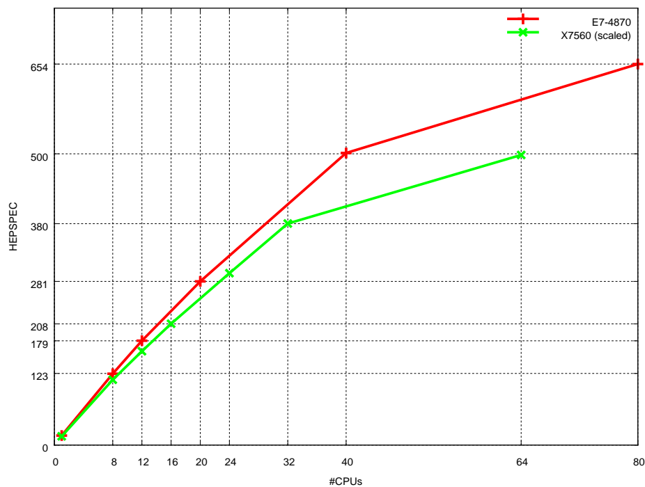
Figure 3. HEPSPEC06 performance comparison “Westmere-EX” E7-4870 vs. “Nehalem-EX” X7560 (frequency scaled). Both systems have SMT on and Turbo mode disabled.
