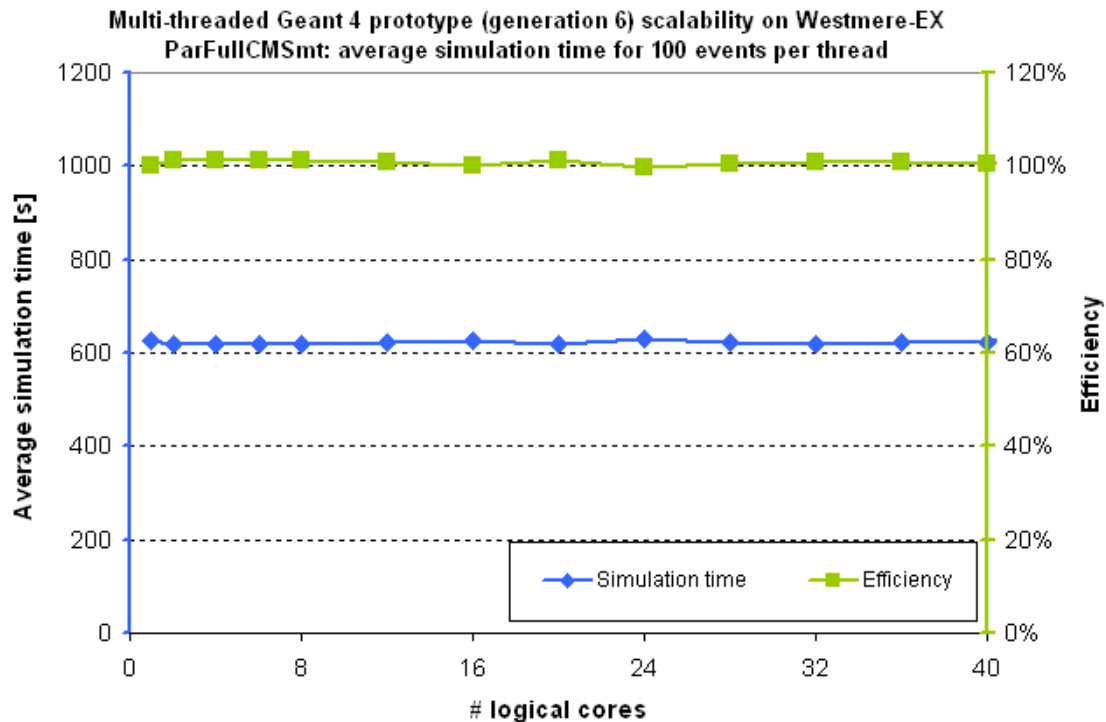
Figure 9. ParFullCMSmt scalability on “Westmere-EX” system (without SMT).
