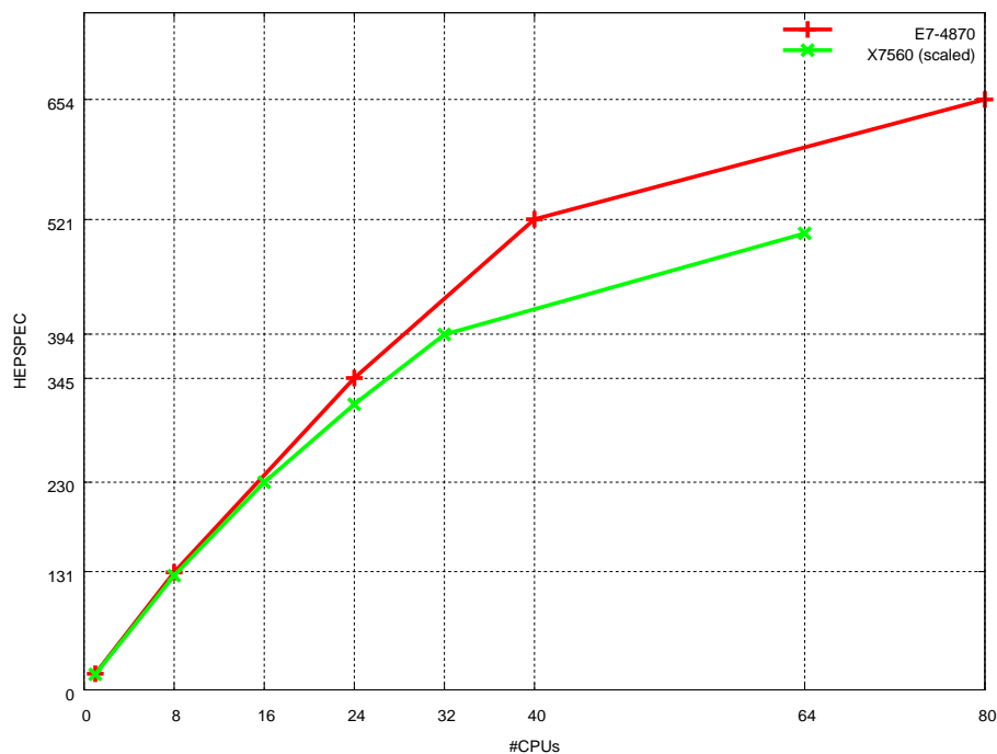
Figure 4. HEPSPC06 performance comparison “Westmere-EX” E7-4870 vs. “Nehalem-EX” X7560 (frequency scaled). Both systems have SMT on and Turbo mode enabled.
