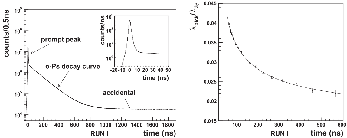
Fig. 2. (Left) Measured o-Ps timing spectrum with the YAP scintillators. (Right) Timing dependence of the pickoff rate. \lambda_{\text{pick}} changes slowly due to the slow thermalization process. Republished with permission from [28].
