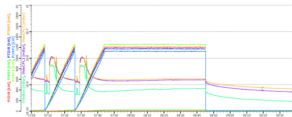
Figure 2: Typical RF conditioning of couplers with vacuum and power measurements.
