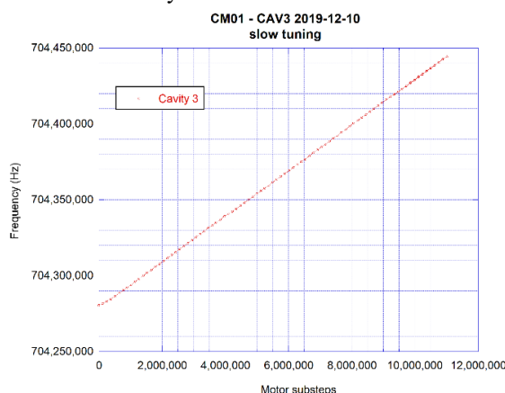
Figure 5: Variation of frequency versus motor sub-steps for CM01 cavity position #3.
