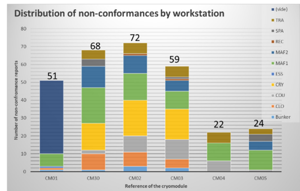
Figure 4: Non-conformances distribution as a function of the cryomodule number and the workstation.
