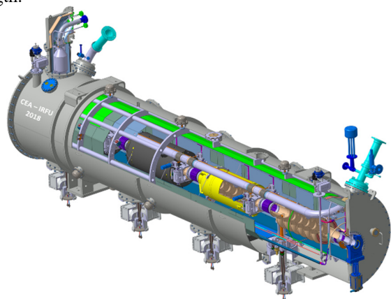
Figure 1: ESS medium-beta cryomodule general layout.
