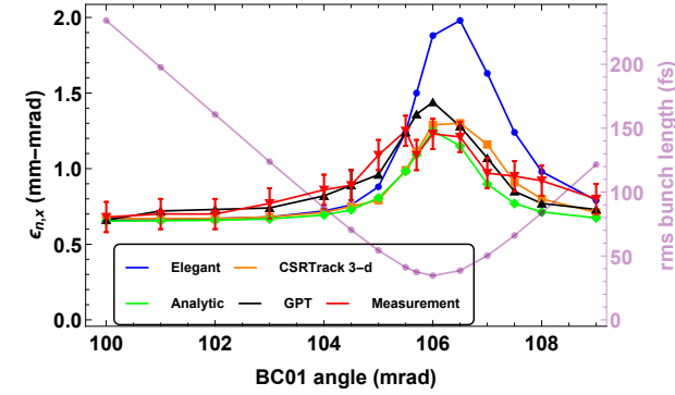
Figure 3: Horizontal emittance as a function of BC01 bending angle, with the corresponding bunch length as simulated by ELEGANT. The analytic results are calculated using Eq. 1.
