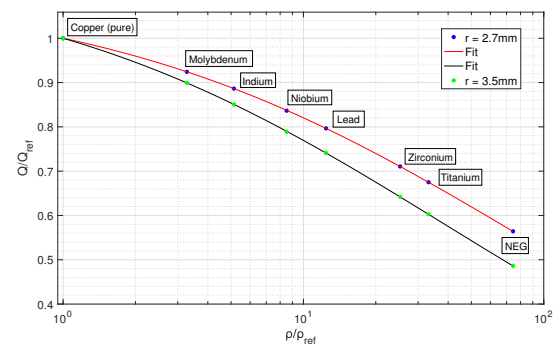
Figure 8: Numerical evaluation of Q-factor variation versus resistivity, normalized to copper for two sapphires.
