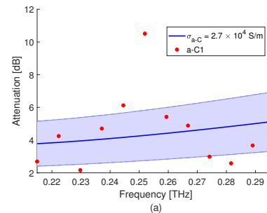
Figure 4: Experimental relative attenuation on the 1 st a-C coated sample (red dots) and best fit curve (blue line).
