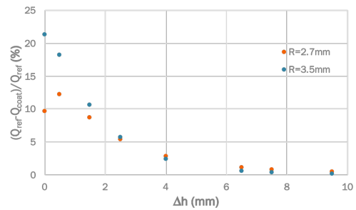
Figure 7: Numerical evaluation of Q-factor relative difference of molybdenum coated copper w.r.t. copper plate (reference) for several distances between dielectric and copper ( \Delta h ) for two sapphires.
