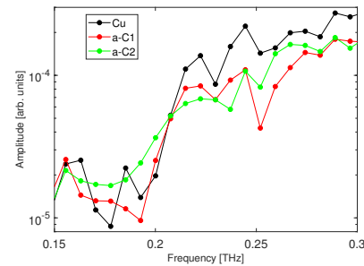
Figure 3: Amplitude transmission data through the waveguide with copper (black curve), with 1 st a-C sample (red curve) and 2 nd a-C sample (green curve).
