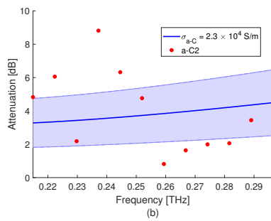
Figure 5: Experimental relative attenuation on the 2 nd a-C coated sample (red dots) and best fit curve (blue line).
