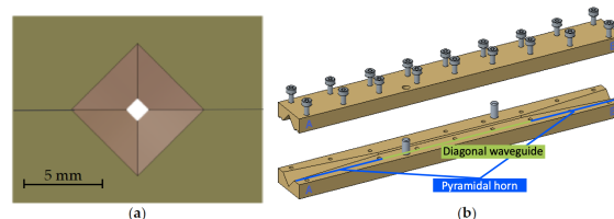
Figure 1: Device consisting of a waveguide with two pyramidal horn antennas. (a) Front view; (b) open view.
