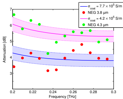
Figure 2: Experimental relative attenuation of 3.8 \mu\text{m} and 4.3 \mu\text{m} NEG coated slabs (red and green dots respectively) and best fit curves (blue and magenta lines respectively).
