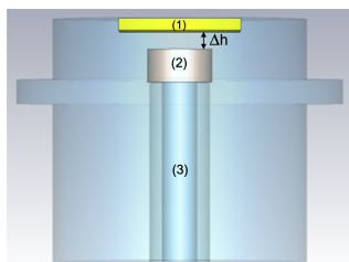
Figure 6: 3D model inside view of the dielectric resonator: 1) copper plate, 2) sapphire puck, 3) quartz hollow holder.
