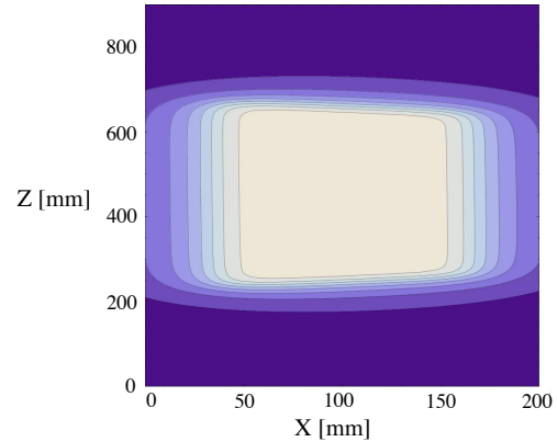
Figure 3: Contour plot of measured magnetic field for the sector magnet shown in Fig. 2. See Fig. 4 for detailed distributions and dimensions.
